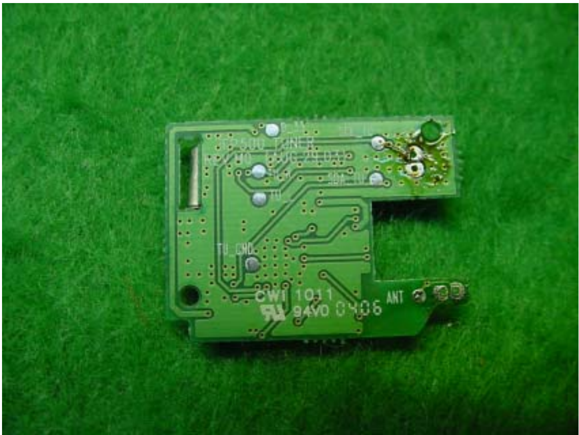
<REAR SIDE OF TUNER BOARD>
