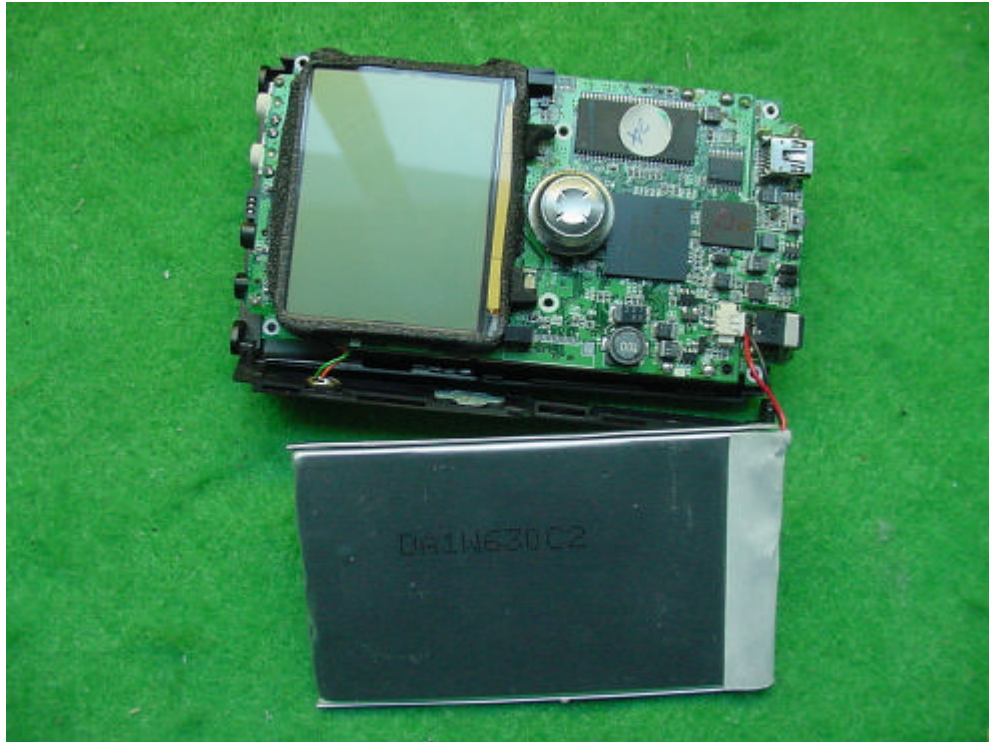
<EUT internal>
