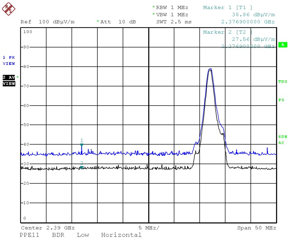
BDR(DH5) Low(Horizontal)
