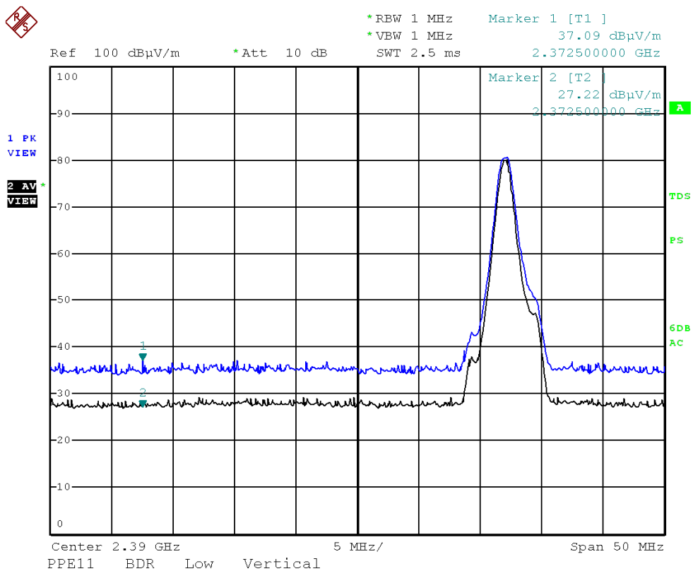
BDR(DH5) Low(VERTICAL)
