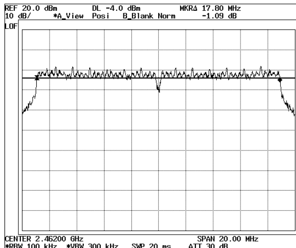
High(2462 MHz)
