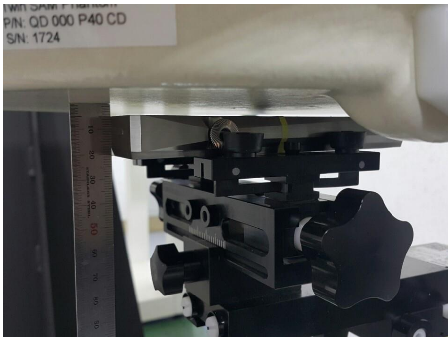
Rear (5 mm)
