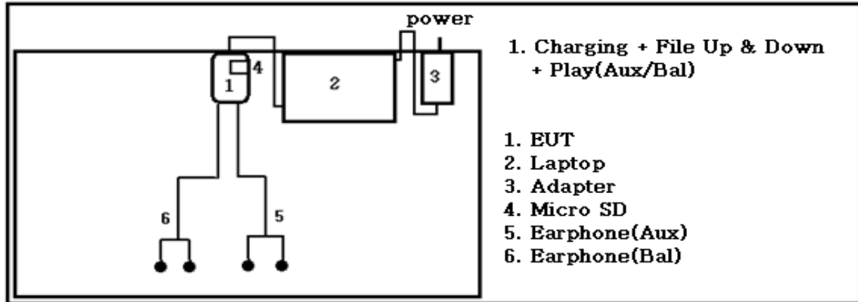
Conducted Emissions
