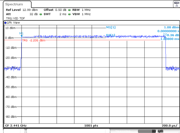
3-DH3
