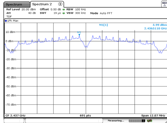
802.11b / 6 ch.
