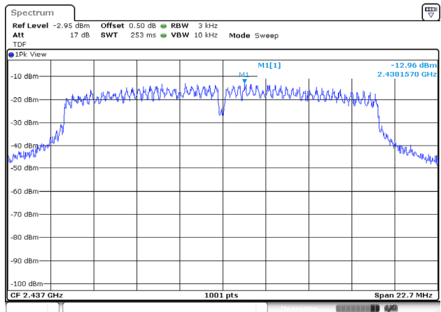
802.11b / 6 ch.
