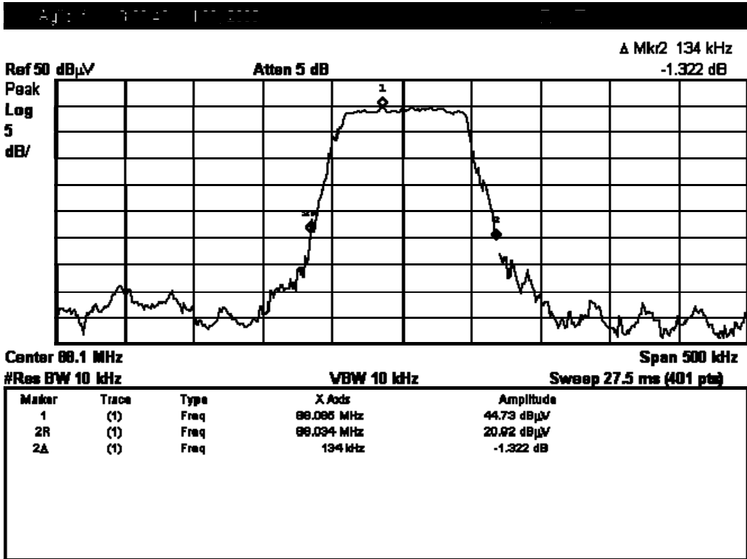
Figure 1: Plot of the Occupied bandwidth Lowest Channel (operating at 88.1 MHz)
