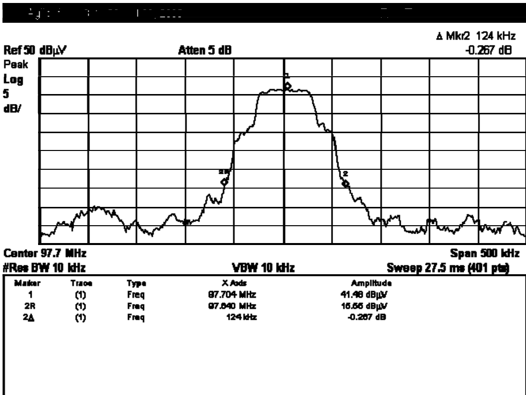
Middle Channel (operating at 97.7 MHz)
