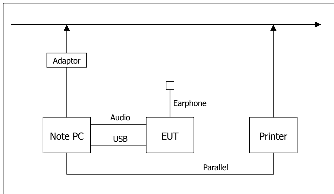
[ System Block Diagram of Test Configuration]
