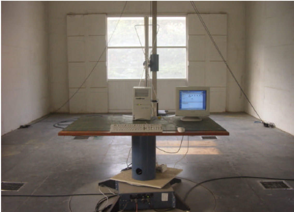
Radiated Emission 30MHz ~ 1000MHz
