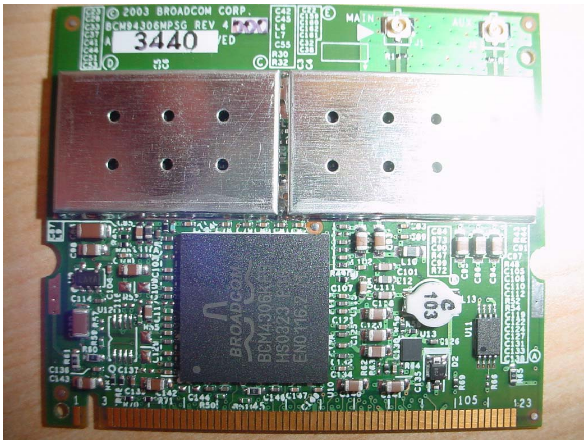
WLAN Model# BCM94306MPSG Top view - shielded
