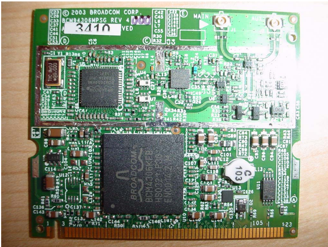
WLAN Model# BCM94306MPSPG Top view - unshielded
