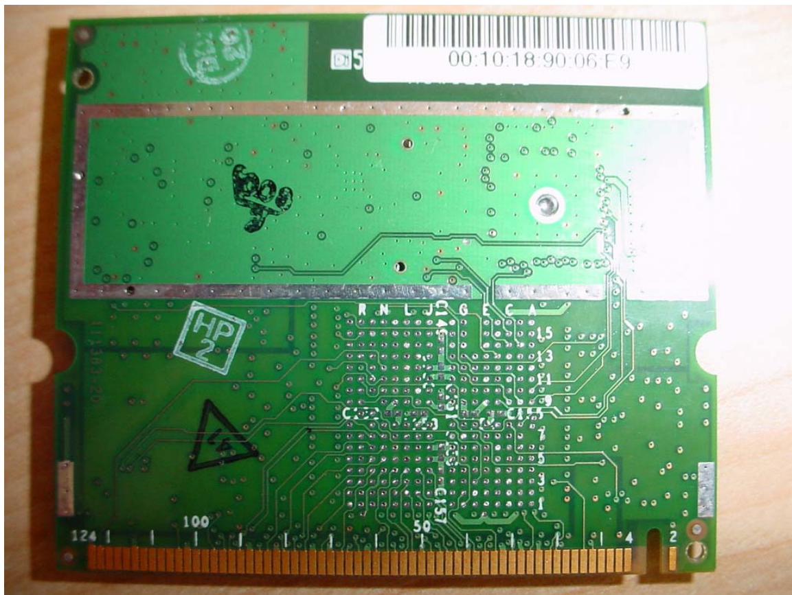
WLAN Model# BCM94306MPSG Bottom view
