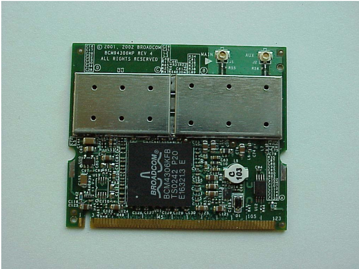
Photo 2. Card top
