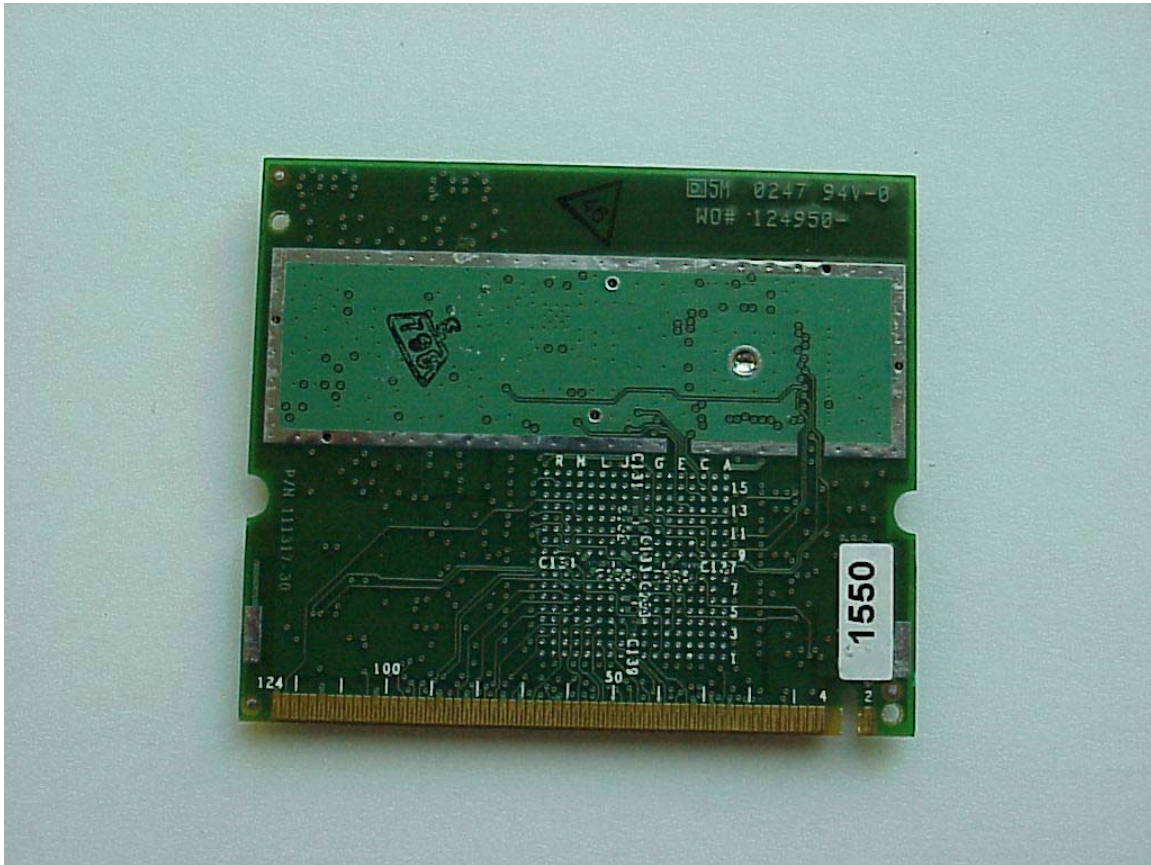
Photo 3. Card bottom
