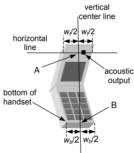
Figure 1b – Handset vertical and horizontal reference lines – "clam-shell"
