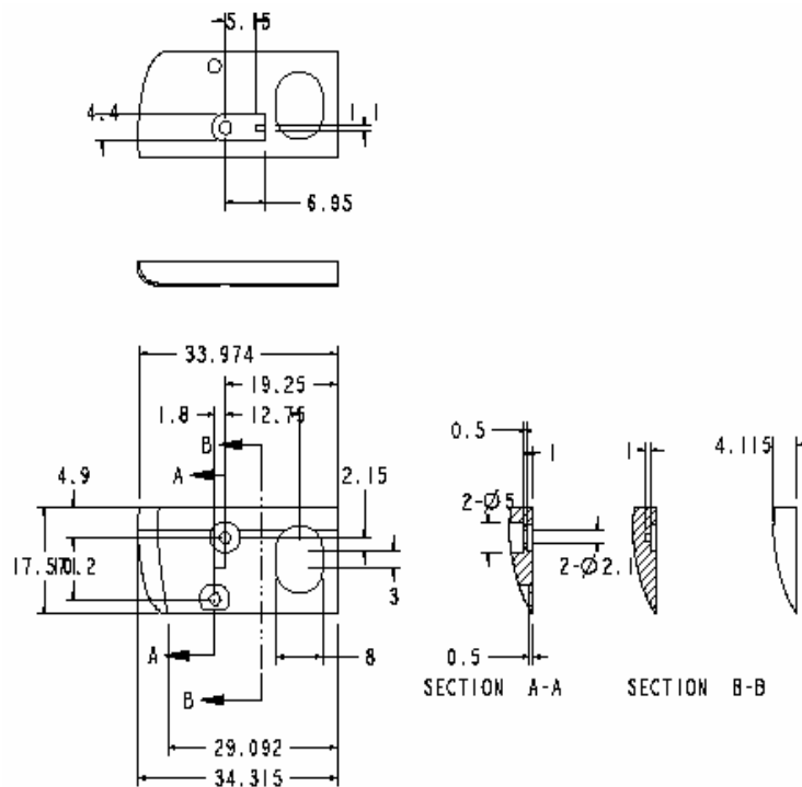
Fig 3.2.2: Cross-section view of left antenna volume
