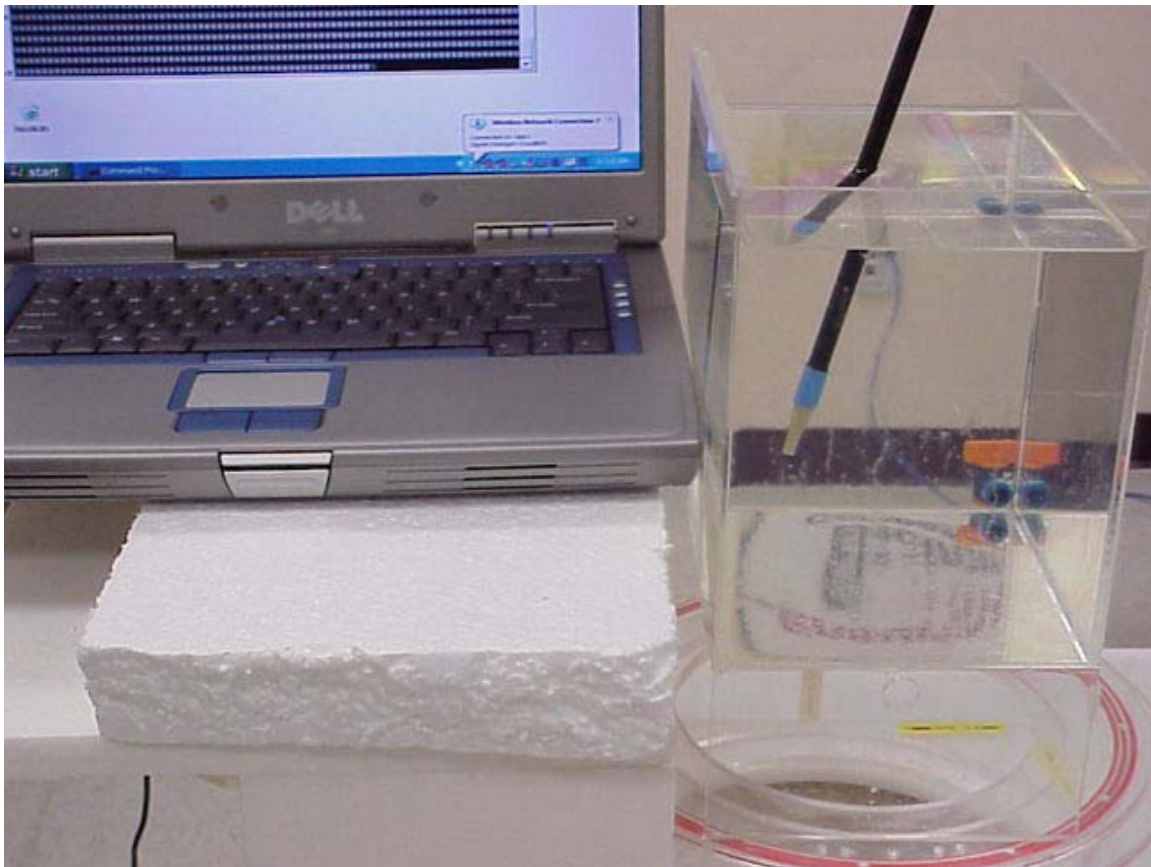
Photo 8. Right antenna bystander position
