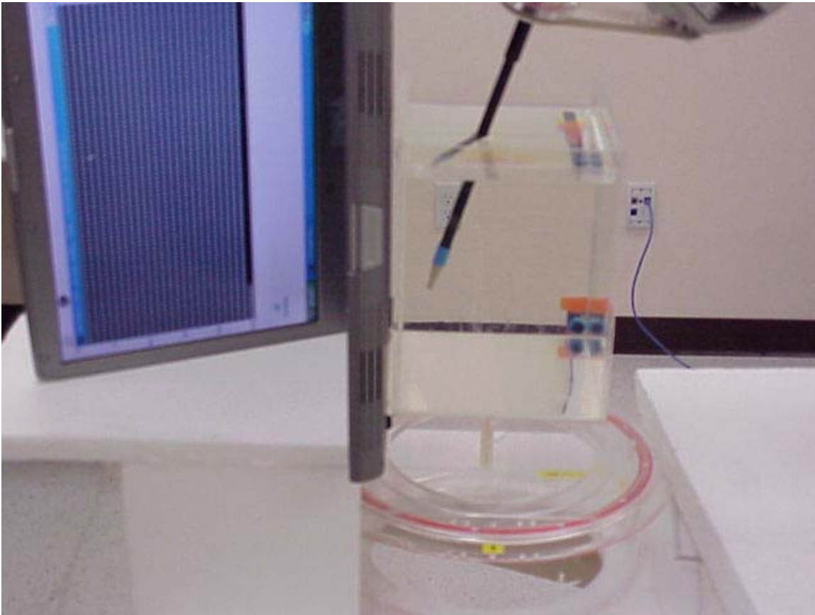
Photo 9. Left antenna lap position
