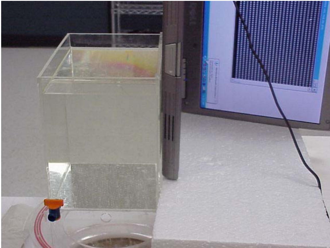
Photo 7. Right antenna lap position
