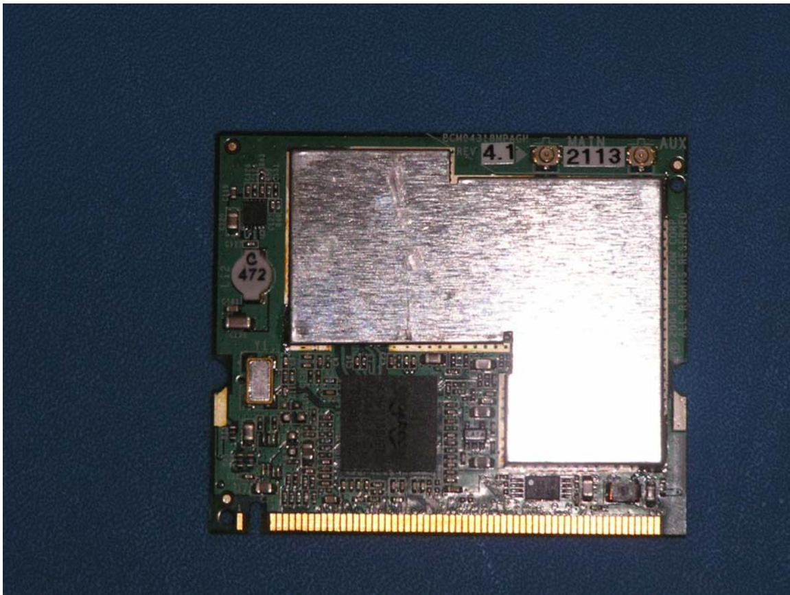
Photo 2. Card top
