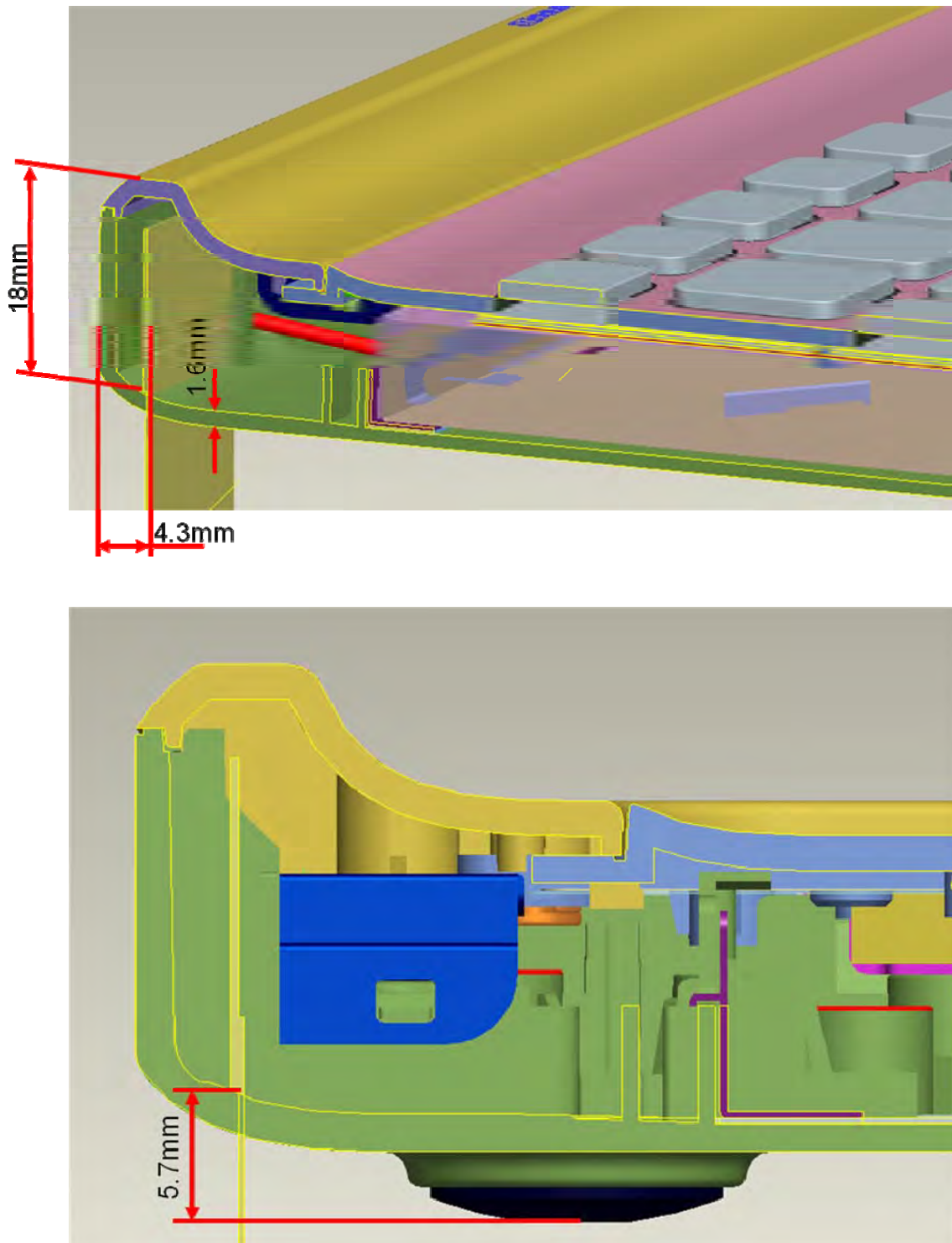
Fig.6 Main Antenna position of EUT
