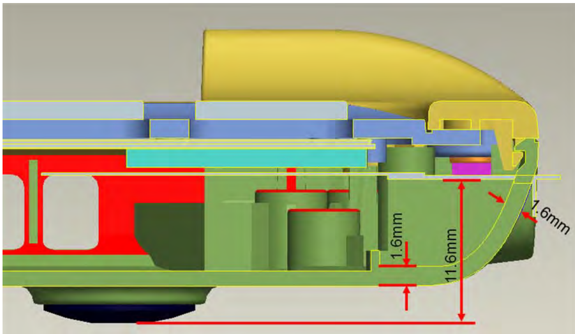
Fig.7 Aux Antenna position of EUT
