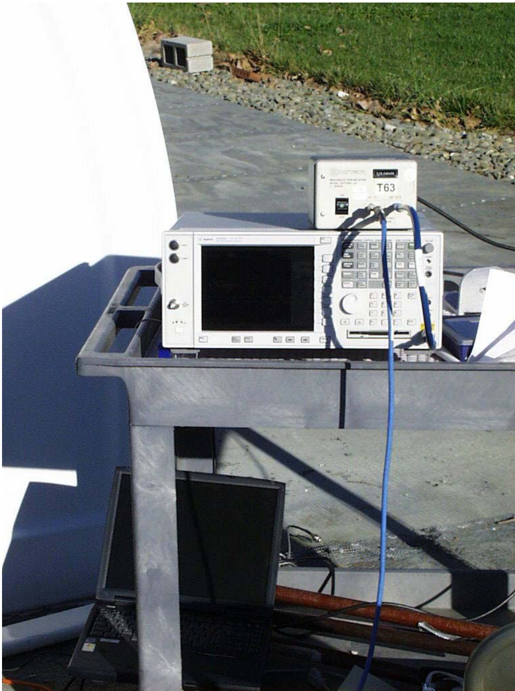
Radiated emissions test equipment
