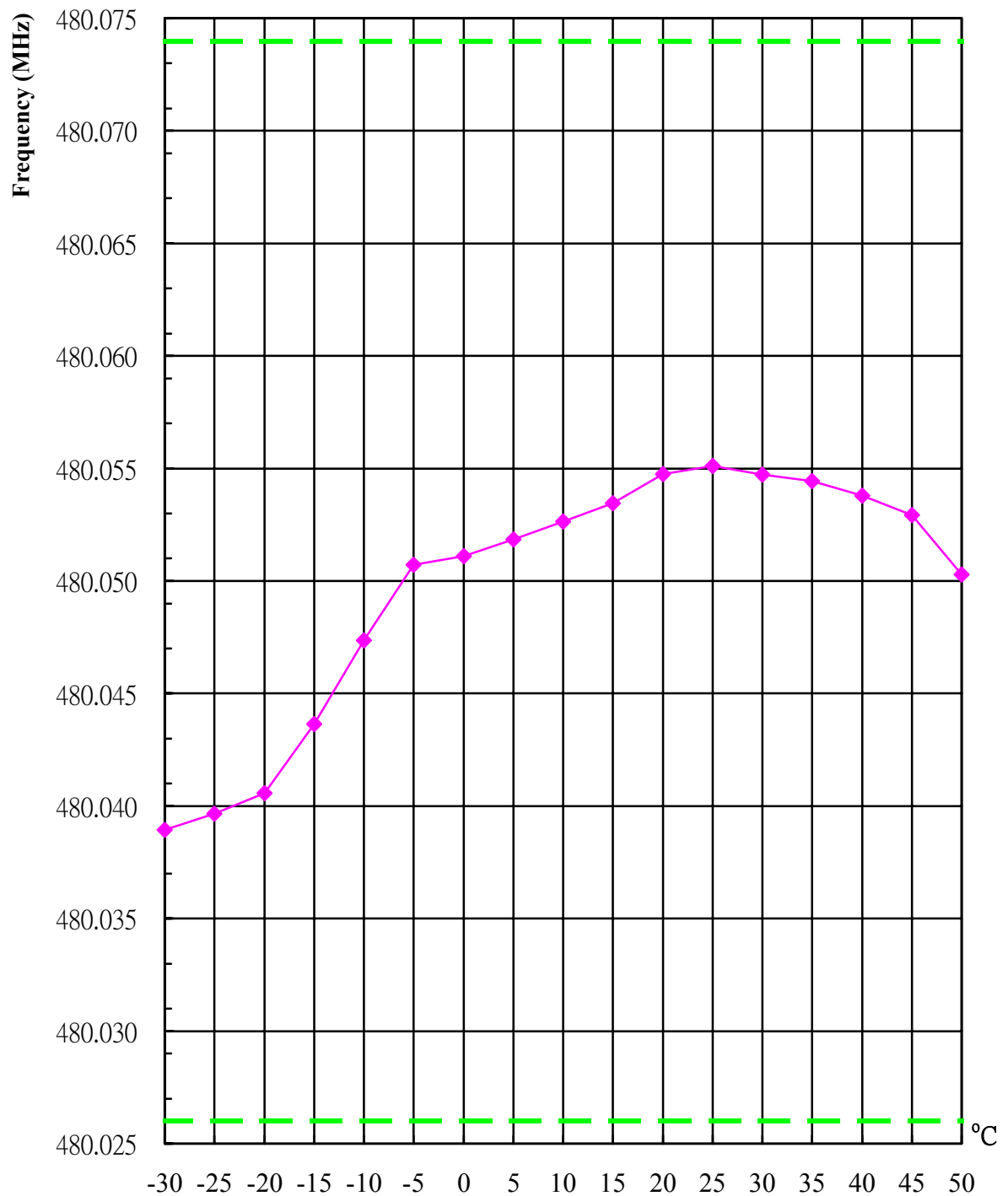
Chart 7.1 Temperatuer Variation Vs. Frequency
