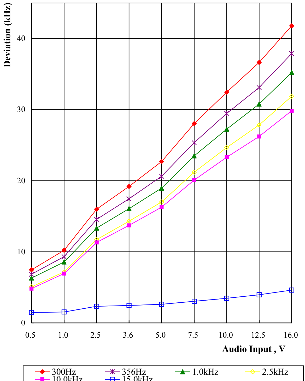
Chart 4.1 Modulation Limiting Measuerment Negative
