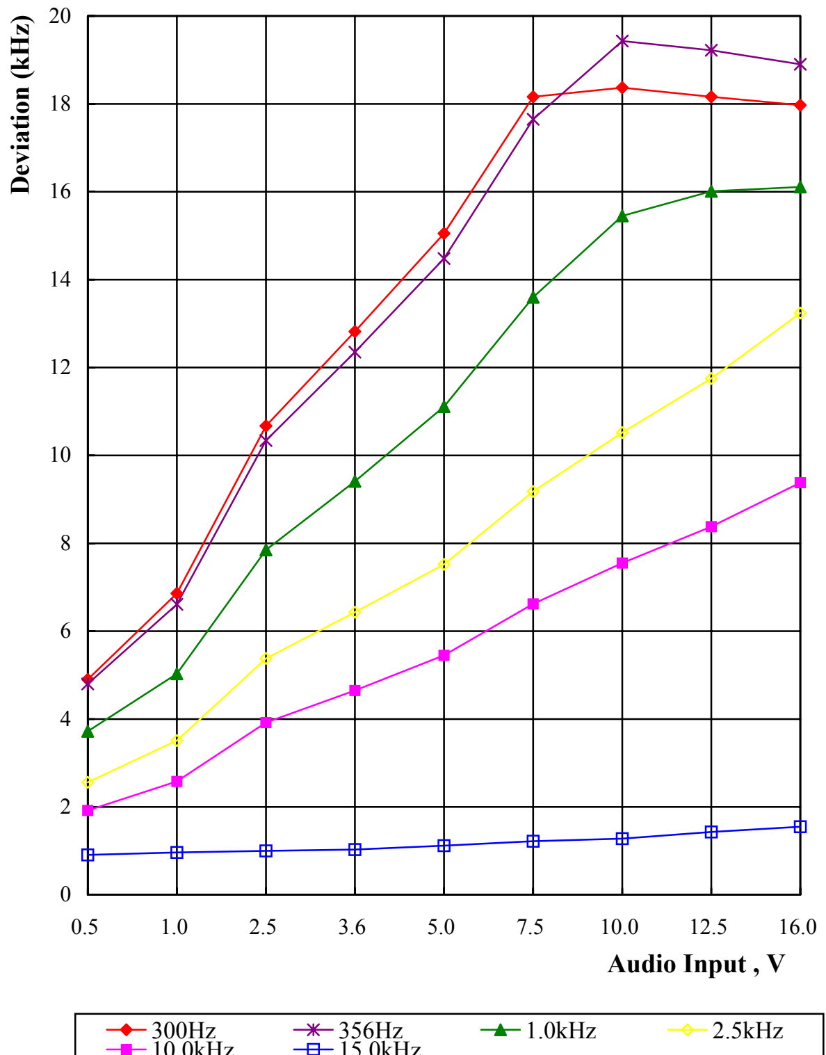
Chart 4.1 Modulation Limiting Measuerment Negative
