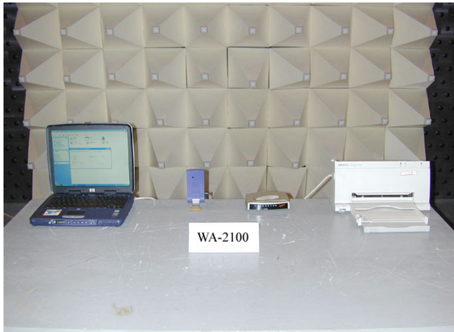
Photo 1: Spurious Test Set-up photo
