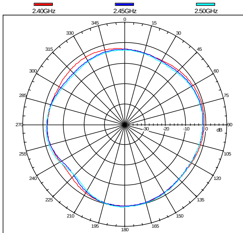
SA2 Dipole Antenna H_Plane
