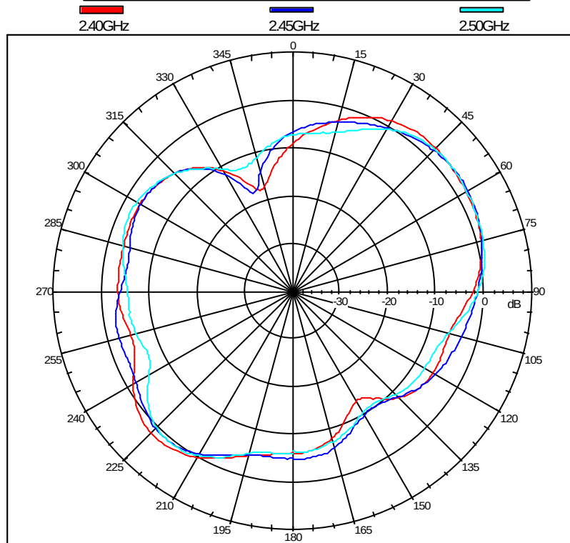
SA2 Dipole Antenna E_Plane
