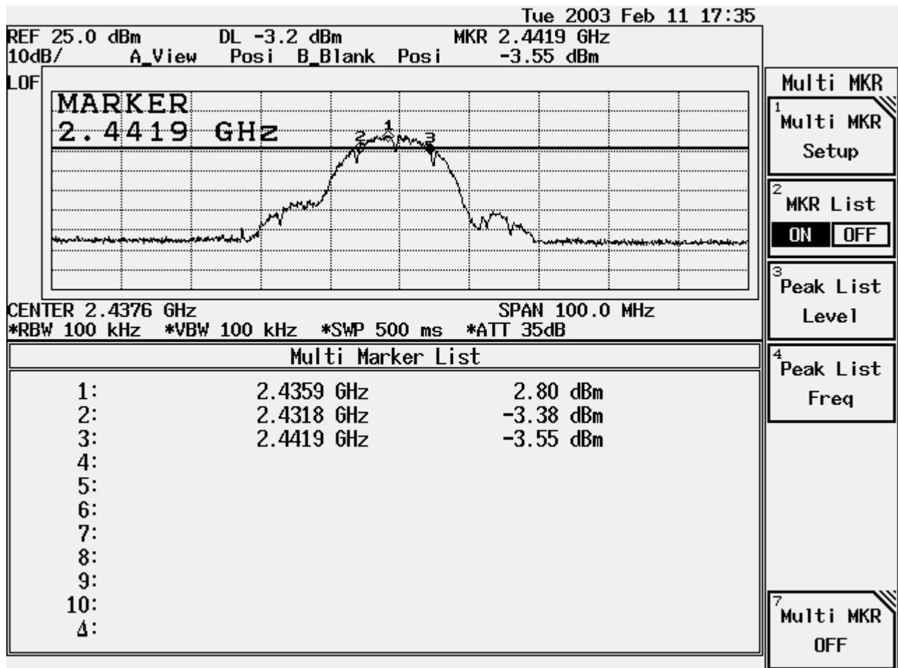
Figure Channel 6: 1Mbps
