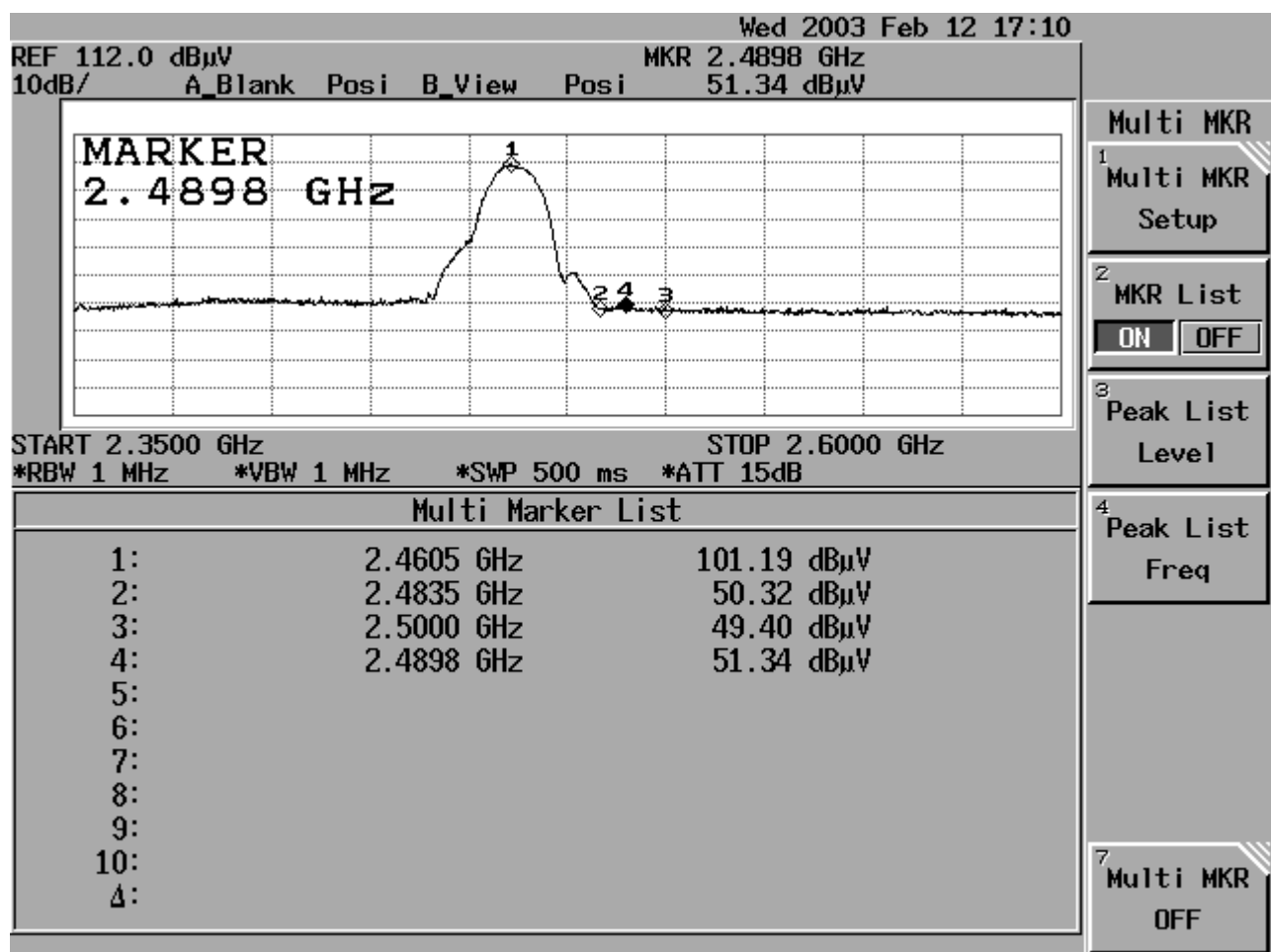
Figure Channel 11: (Vertical)
