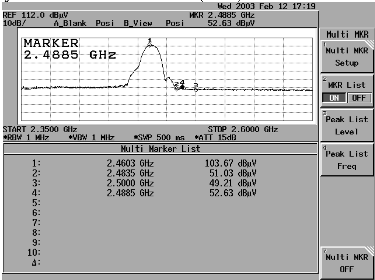
Figure Channel 11: (Horizontal)
