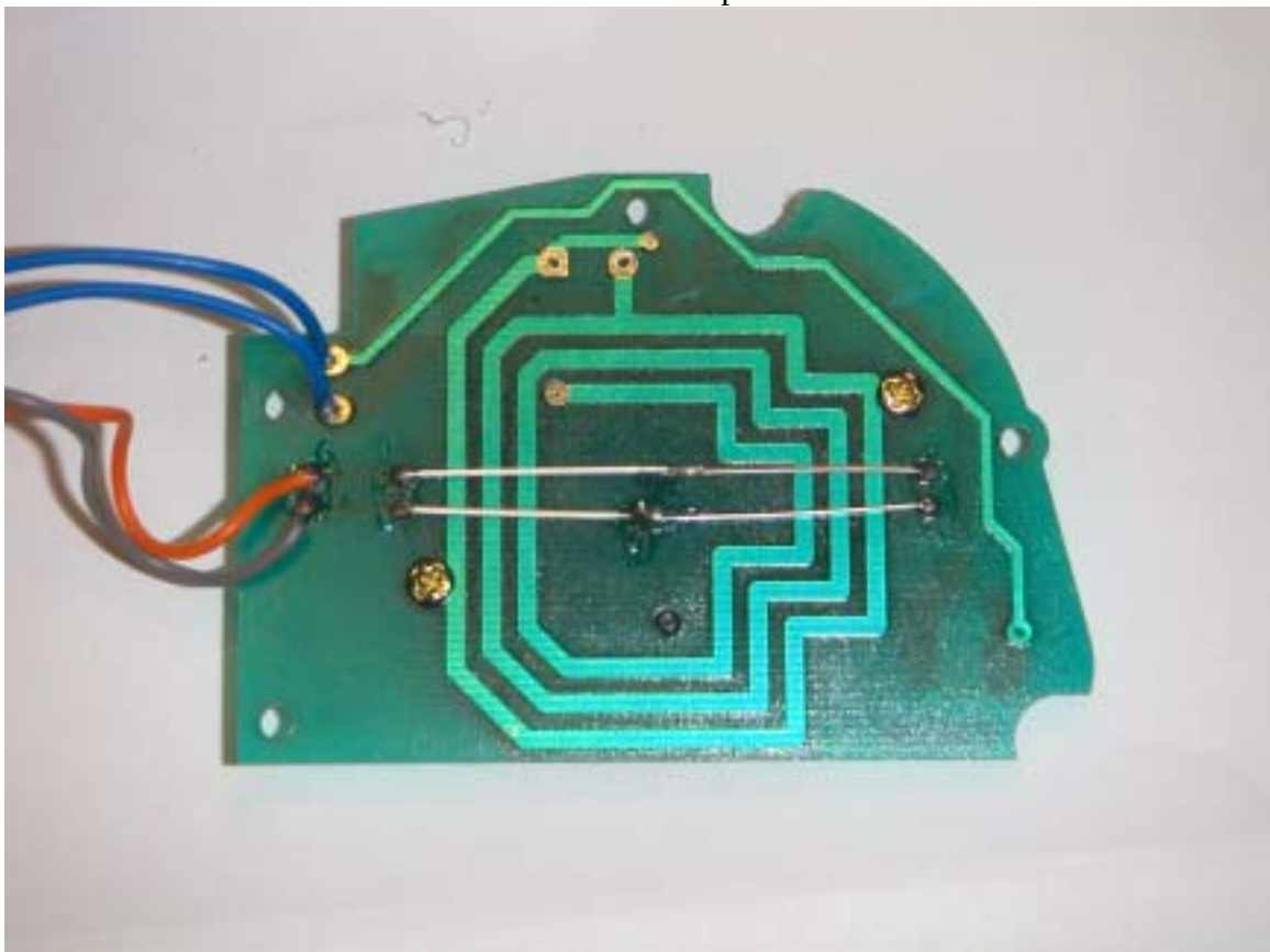
Antenna PCB – Bottom side
