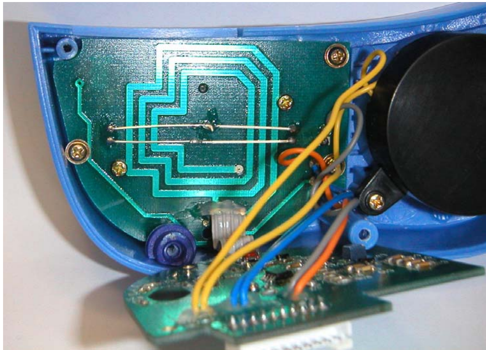
Antenna Board – Bottom Side
