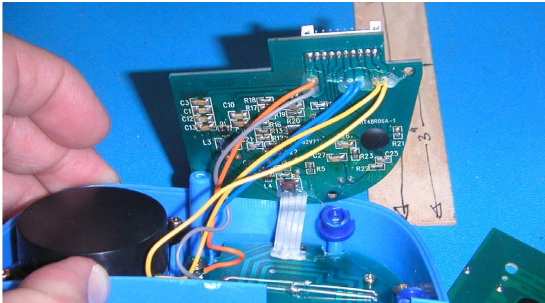
Scanner Board – Top (component) Side Showing Connection To Antenna Board
