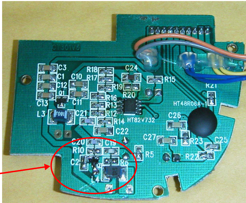
Circuit Board – top side
