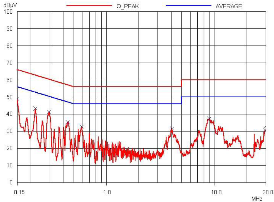
HOT LINE
