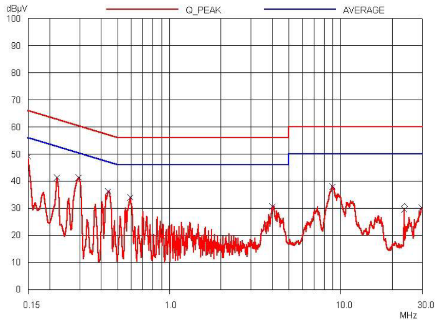
NEUTRAL LINE
