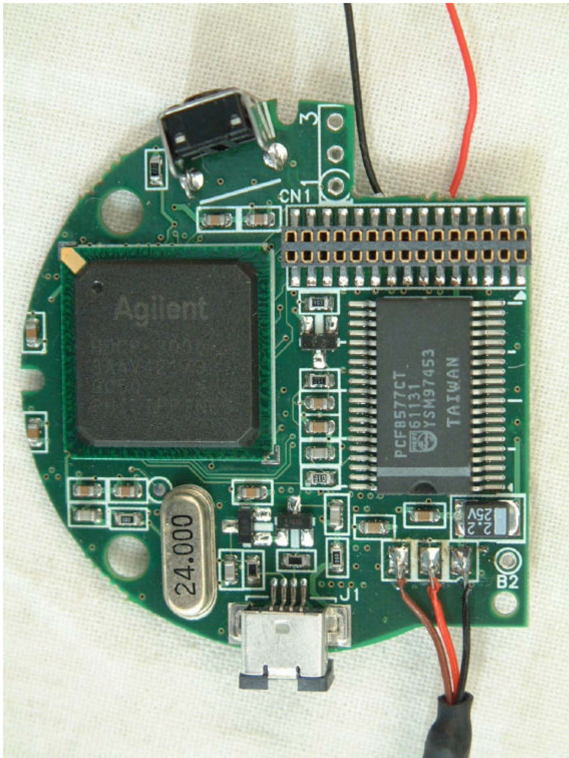
<REAR VIEW OF MAIN-UP BOARD>
