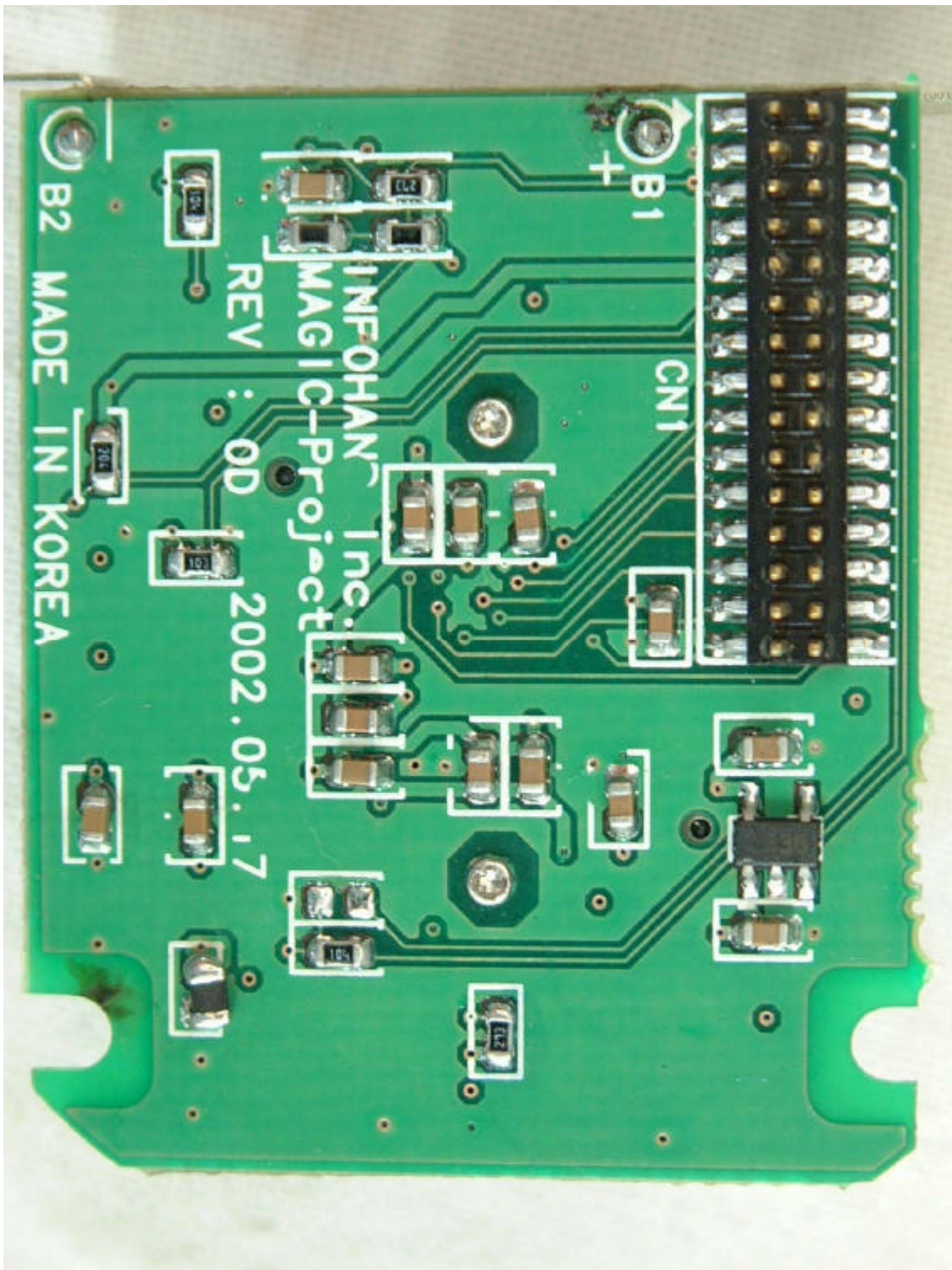
<REAR VIEW OF MAIN-DOWN BOARD>
