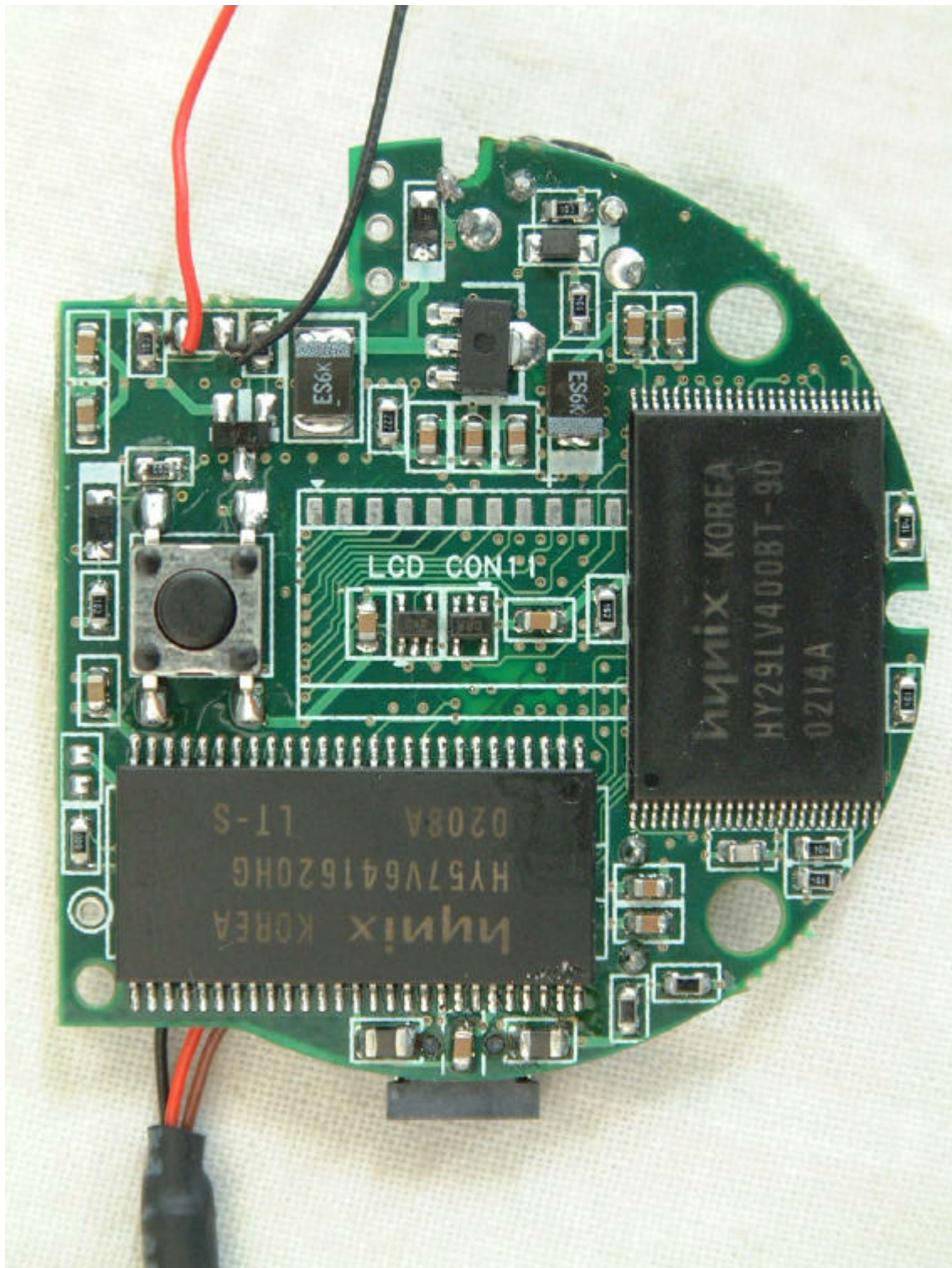
<FRONT VIEW OF MAIN-UP BOARD>
