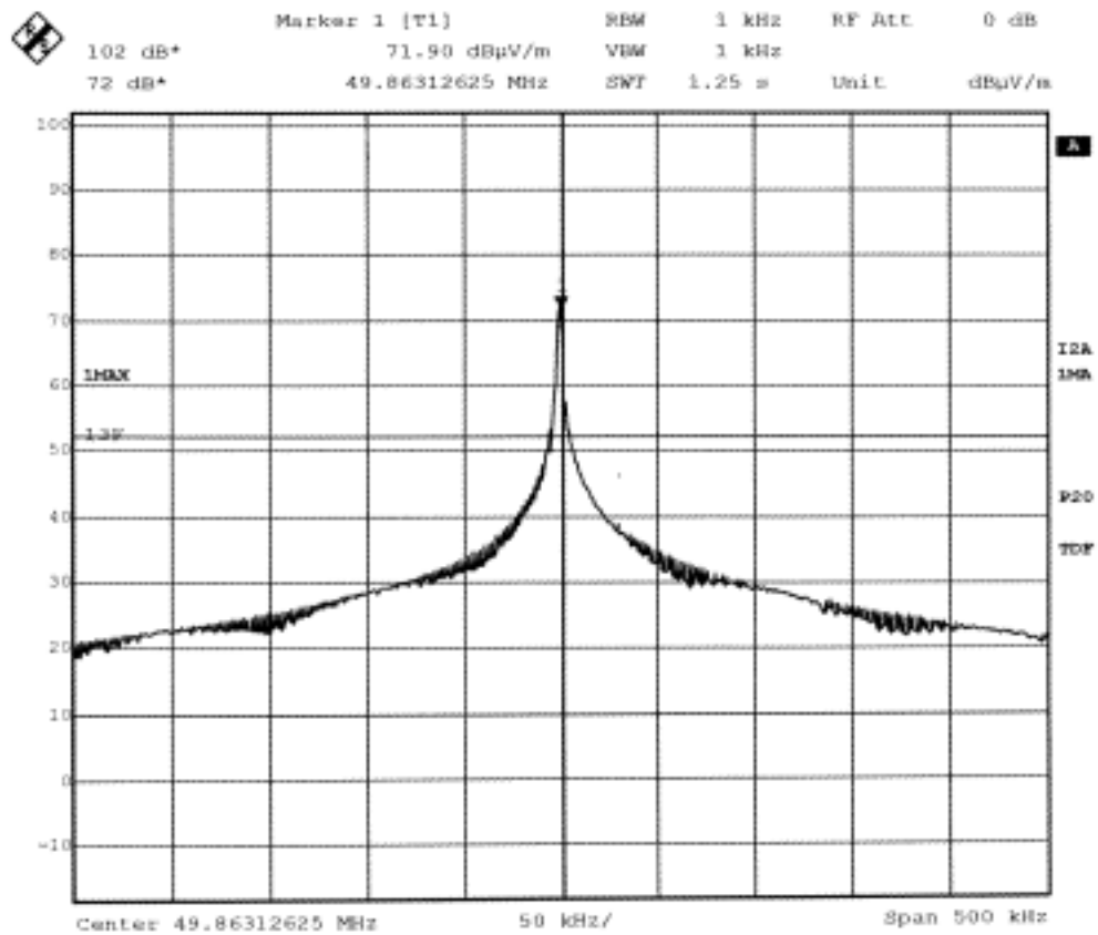
Bandwidth plot at RBW 1kHz, VBW 1kHz, Span 500kHz
