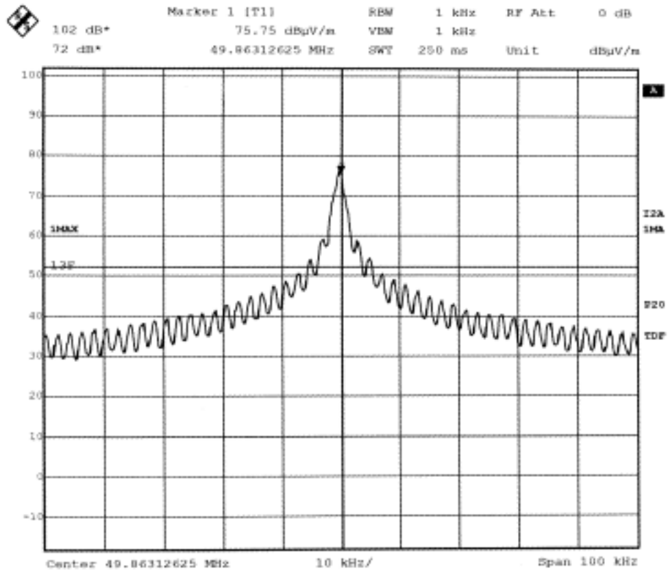
Bandwidth plot at RBW 1kHz, VBW 1kHz, Span 100kHz
