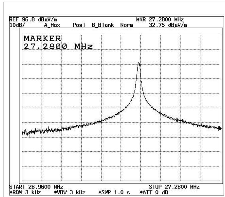
Bandwidth Plot
