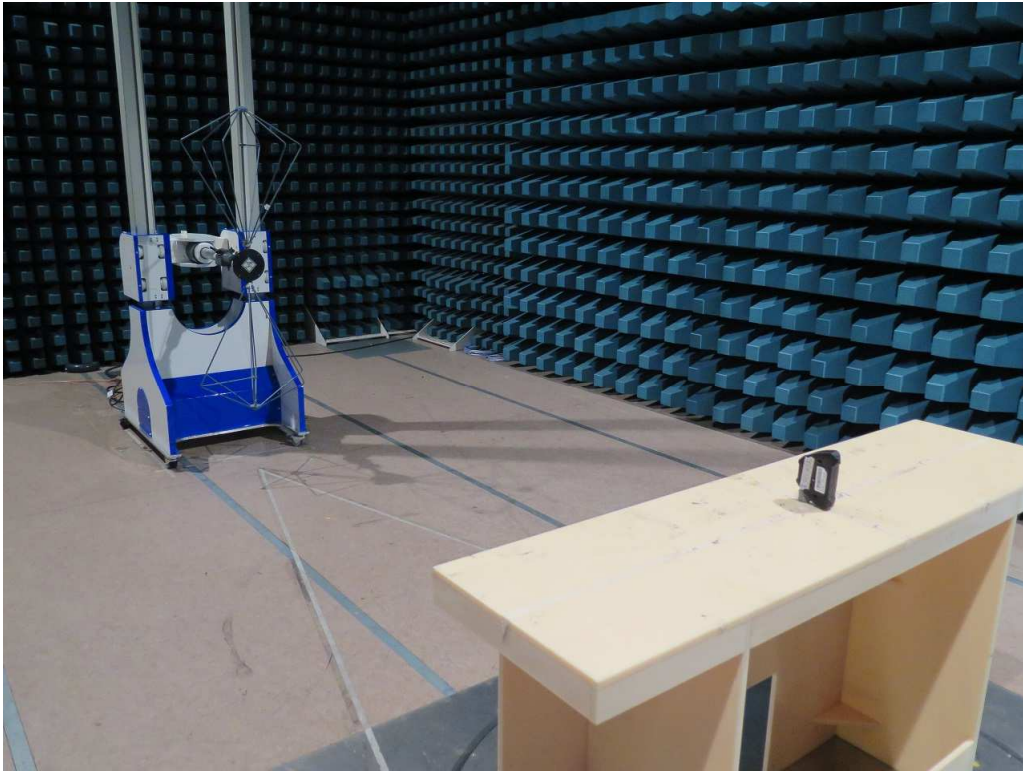
Front view (30MHz – 200MHz)
