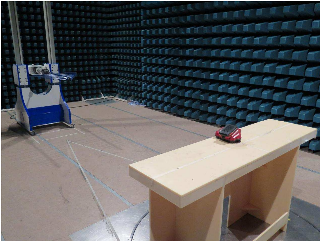
300MHz – 1GHz (Front view, charging)
