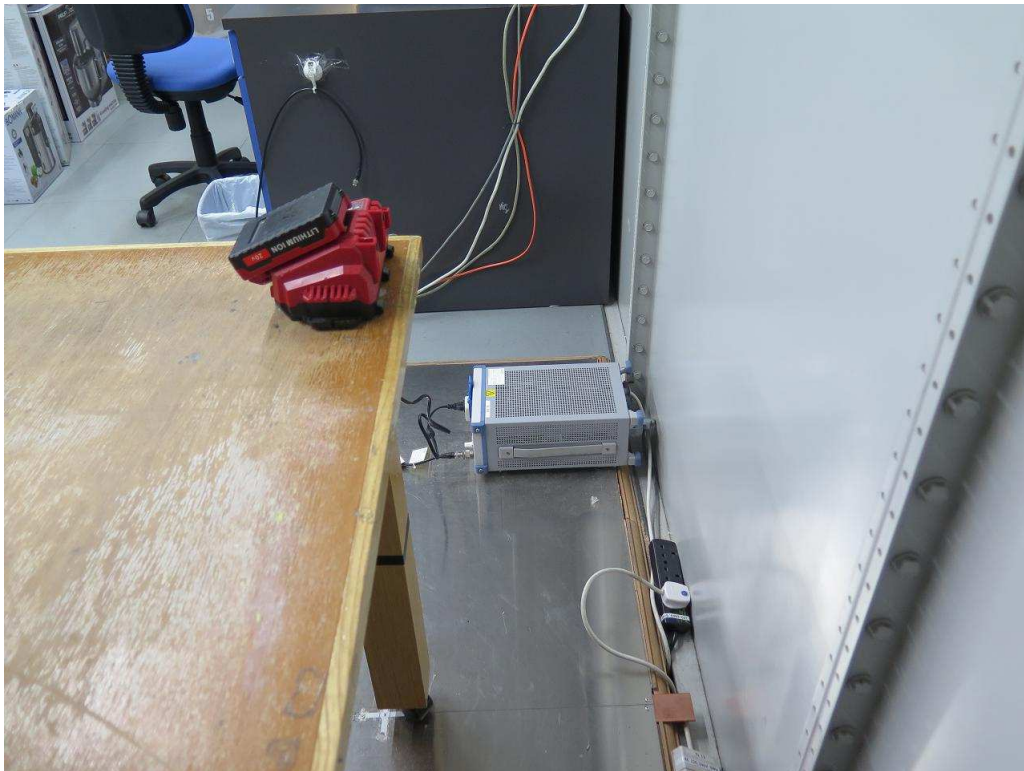
Line-conducted emission (rear view, charging)
