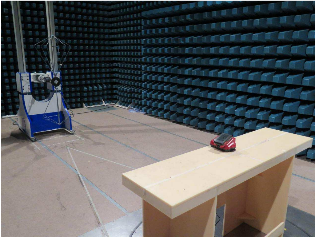
30MHz – 300MHz (Front view, charging)
