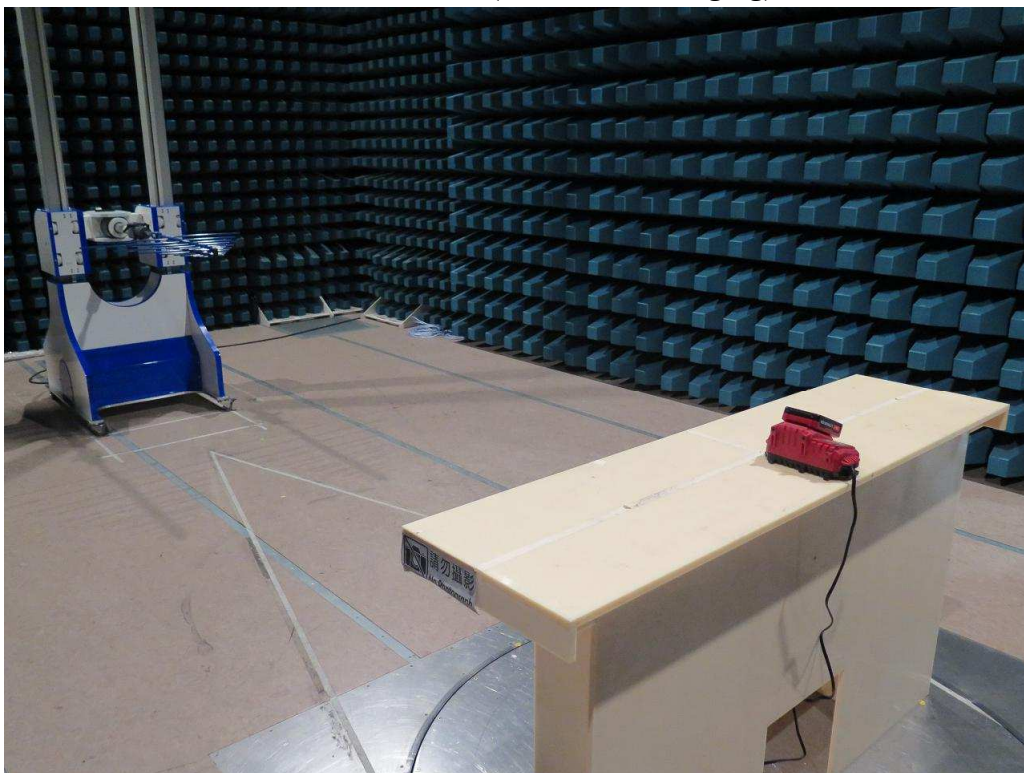
300MHz – 1GHz (Rear view, charging)
