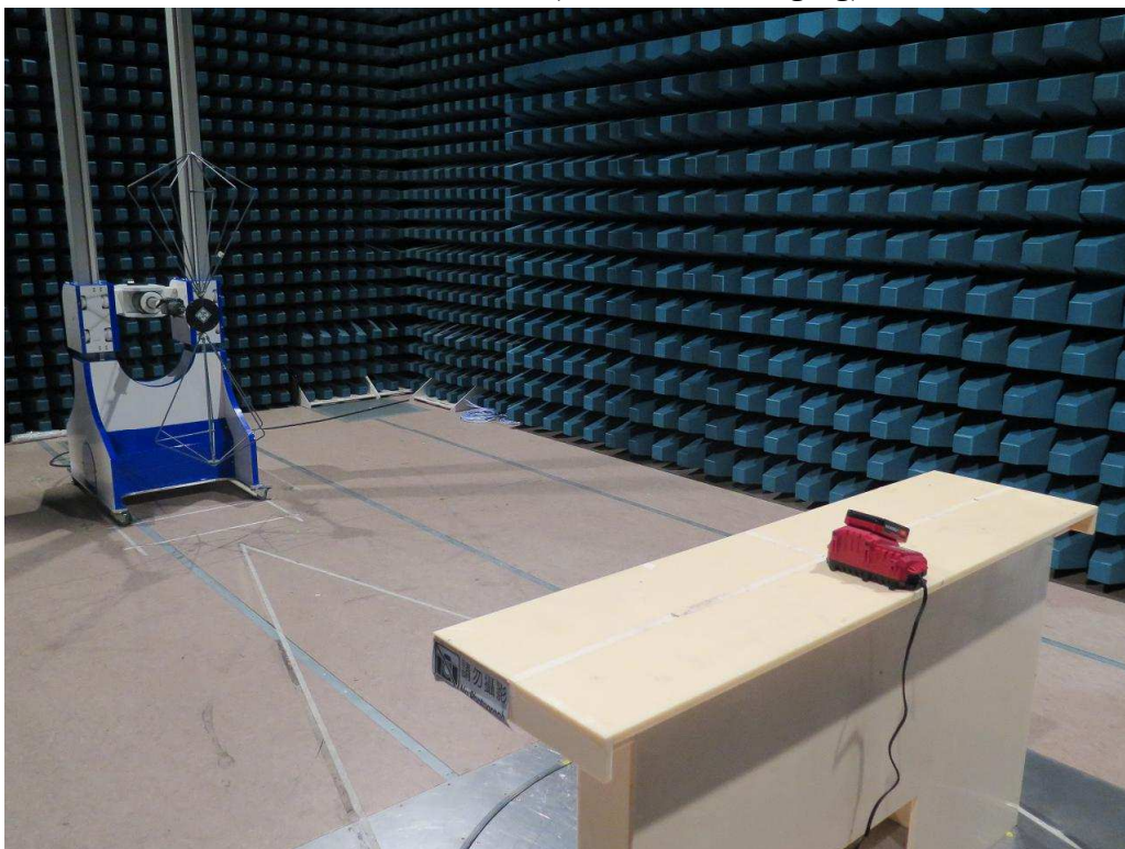
30MHz – 300MHz (Rear view, charging)
