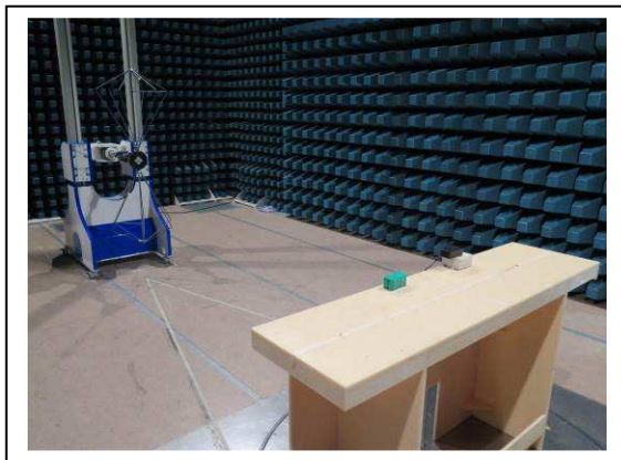
30MHz – 300MHz (Charging, front view)
