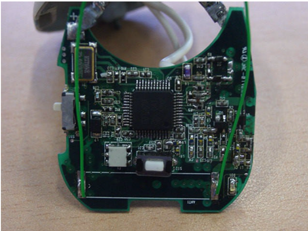
<ear main board front>
