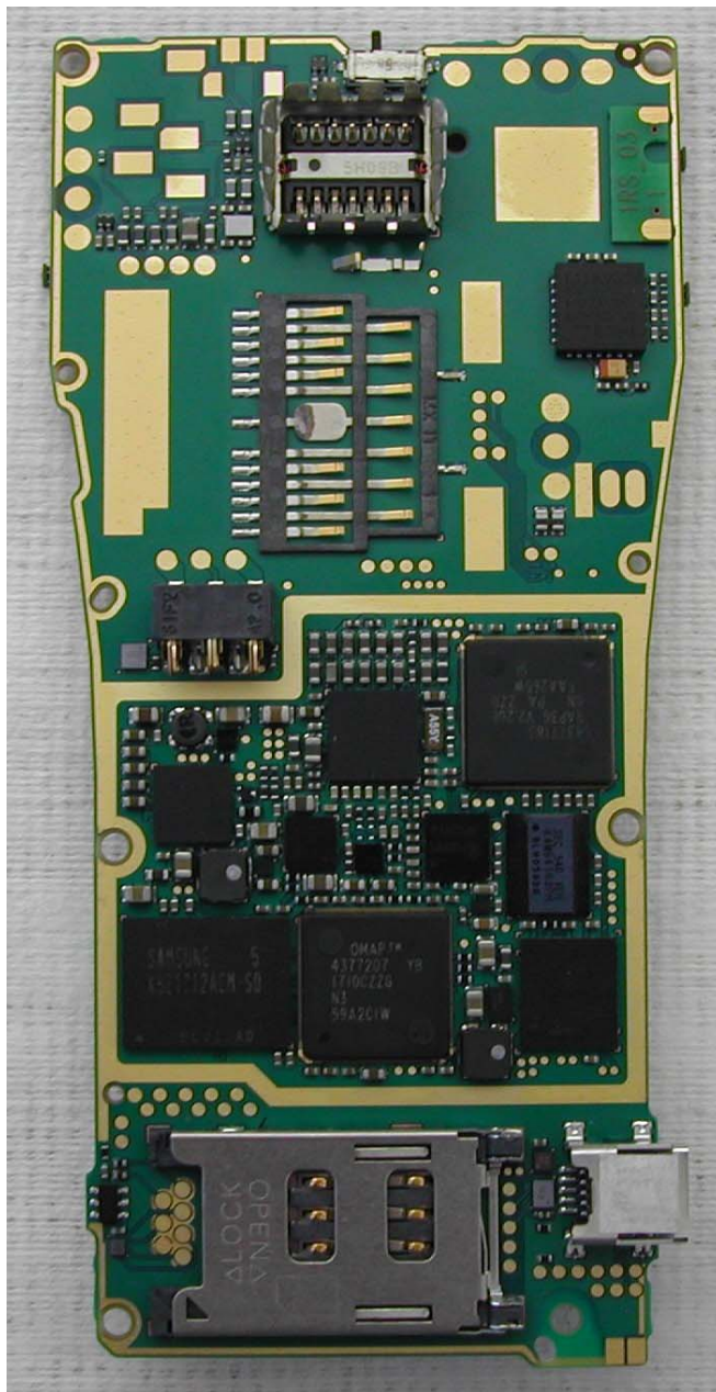
Fig 4 – PCB – Back view
