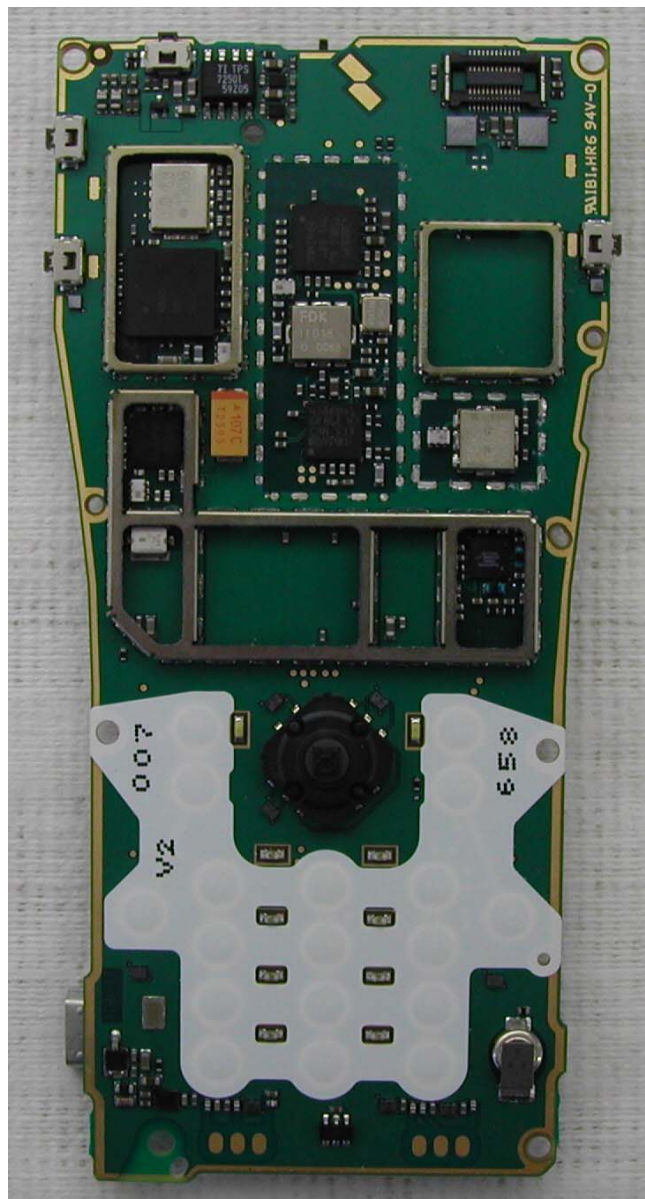
Fig 2 – PCB – Front View (shields removed)
