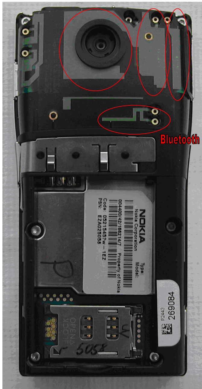
Fig 6 – Back showing antennas
