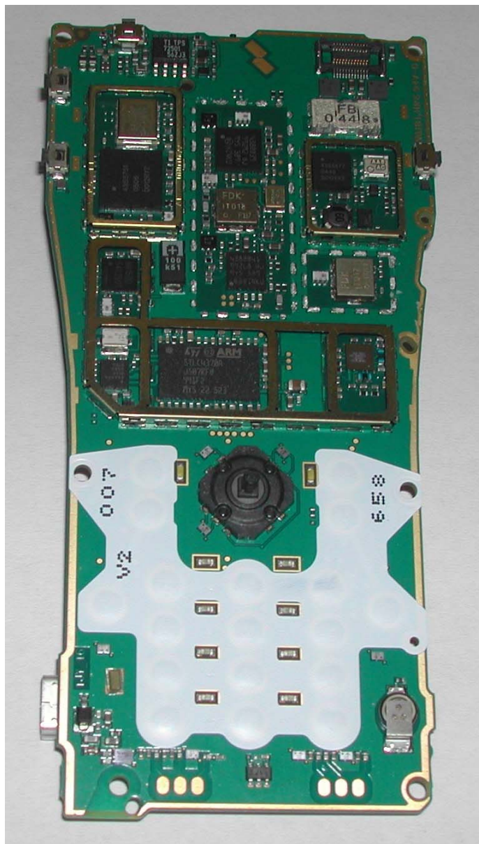
Fig 2 – PCB – Front View (shields removed)
