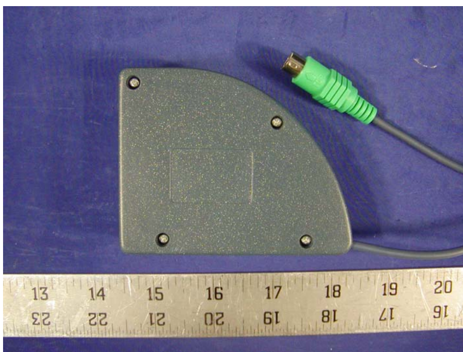
Receiver Chassis - Bottom View
