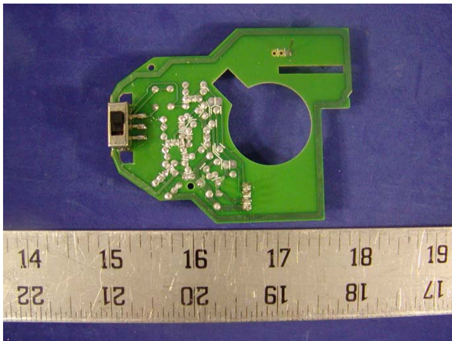
Transmitter Main Board - Solder View
