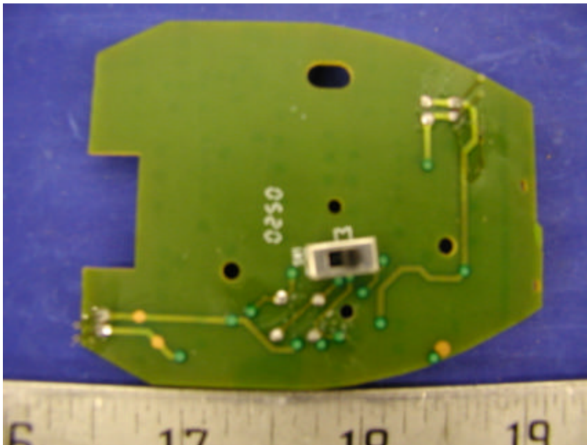
Transmitter Main Board – Solder View 2
