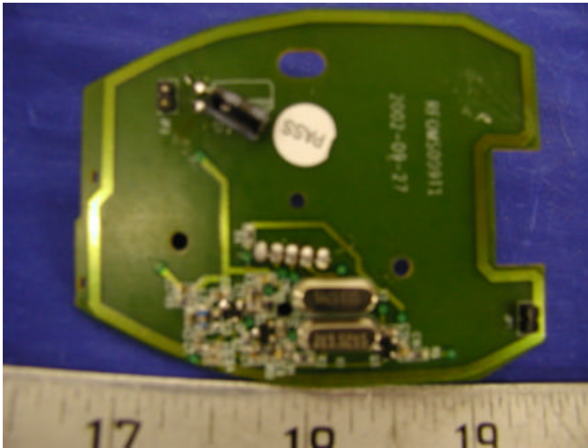
Transmitter Main Board – Component View 2
