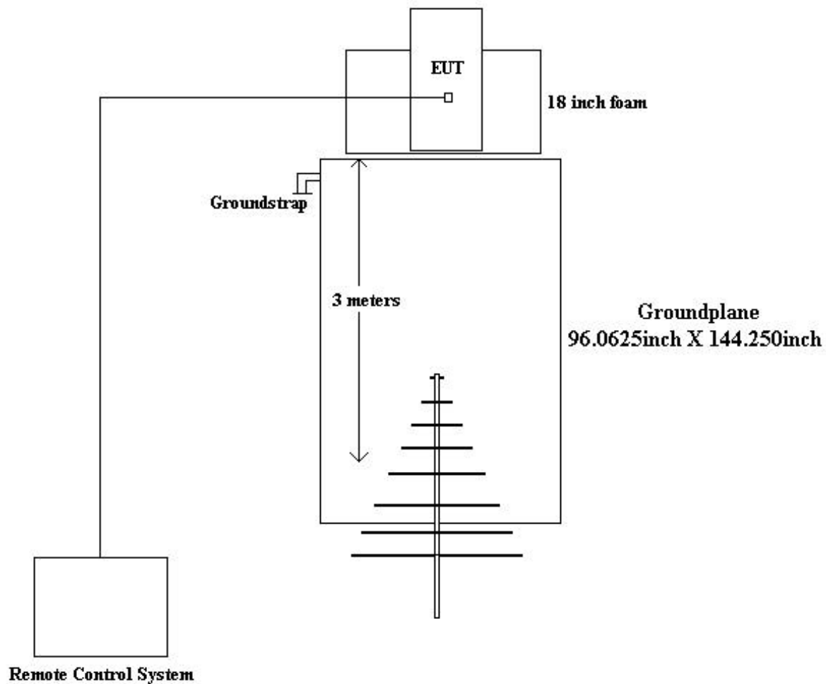
FIGURE 1.3-1 TEST SETUP BLOCK DIAGRAM (M/N 4108)
