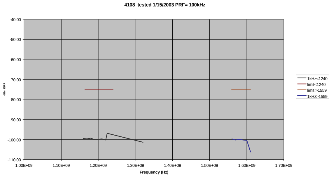
FIGURE 4.3-1 4108F RMS (GPS; RBW=1kHz)
