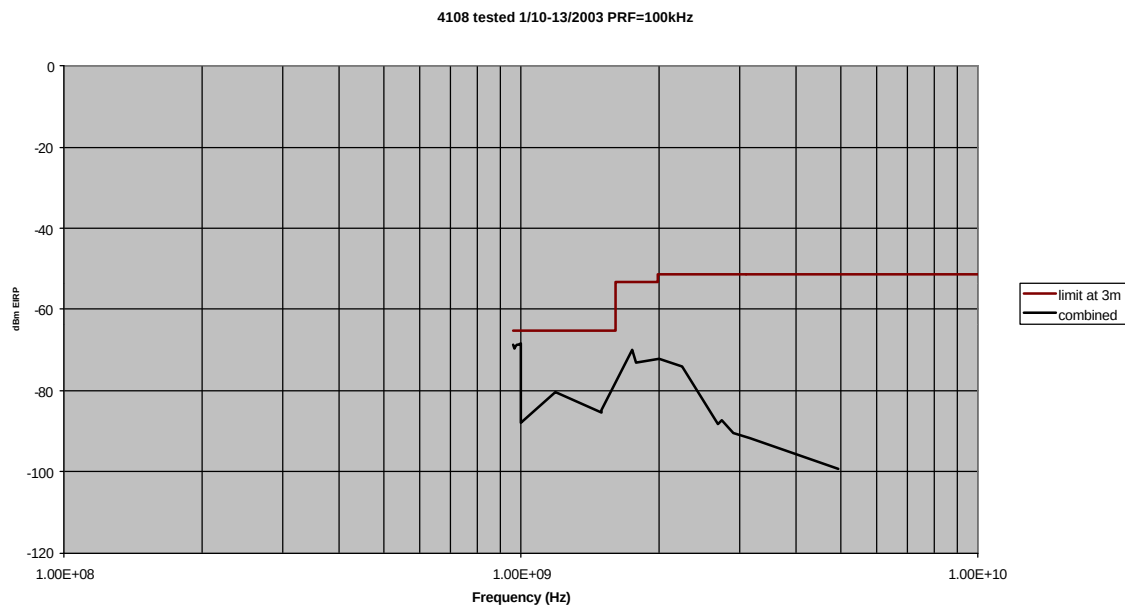
FIGURE 4.2-1 4108F RMS (RBW=1MHz)
