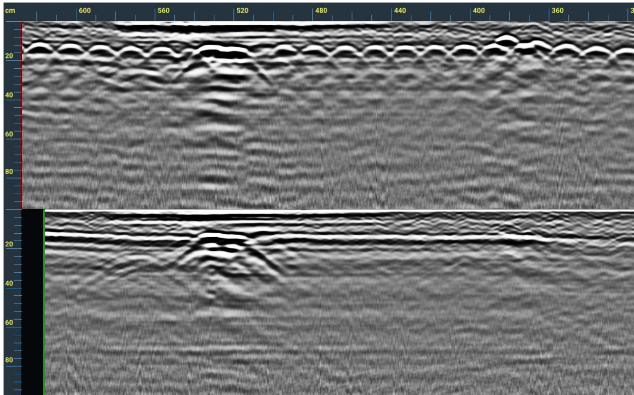
Flex NX Collection Mode displaying Stacked profiles. The top profile (standard orientation) exhibits shallow wire mesh and a possible conduit bank. In the bottom profile (cross-polarized) the wire mesh is not visible, and the removal of hyperbolic tails reveals more details about the conduit bank and a previously obscured target to its left.
