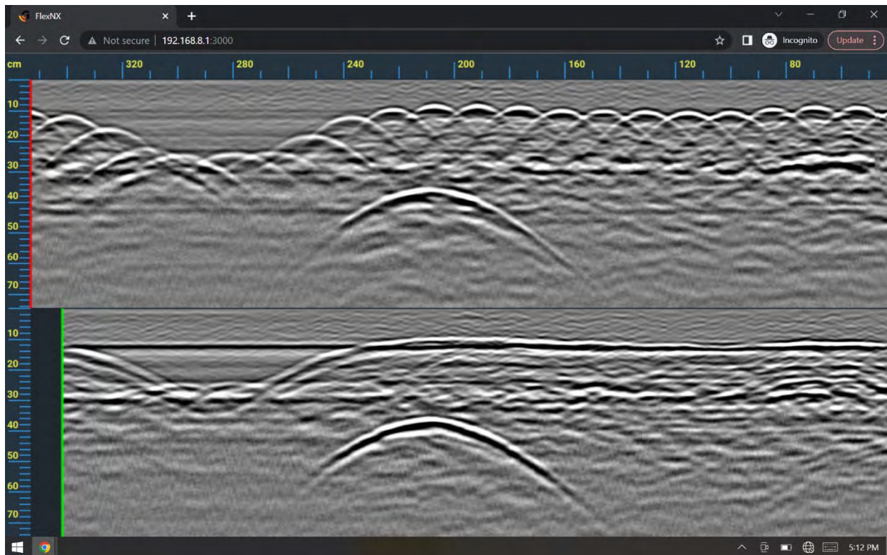
Flex NX data collection mirrored to a tablet. Data mirroring will appear similarly on most devices.
