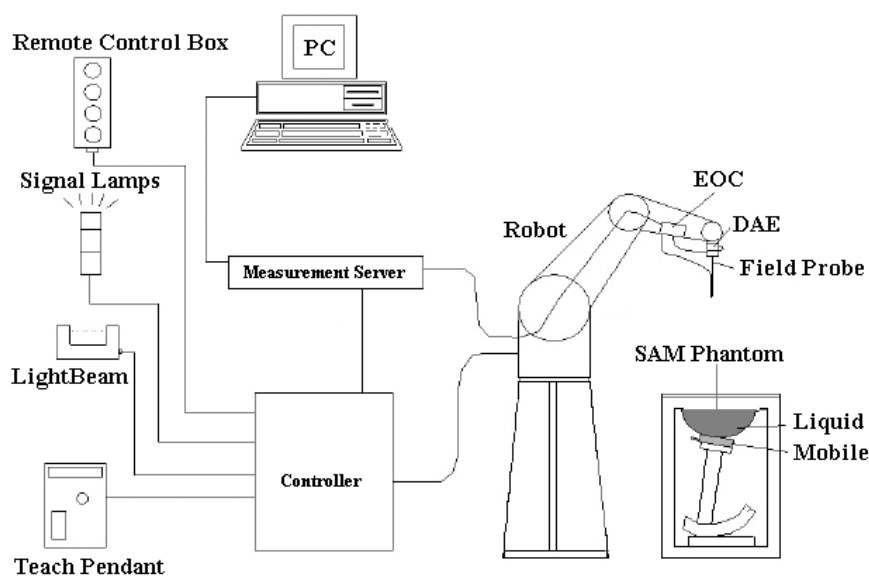
Fig. 4: The DASY4 measurement system.
