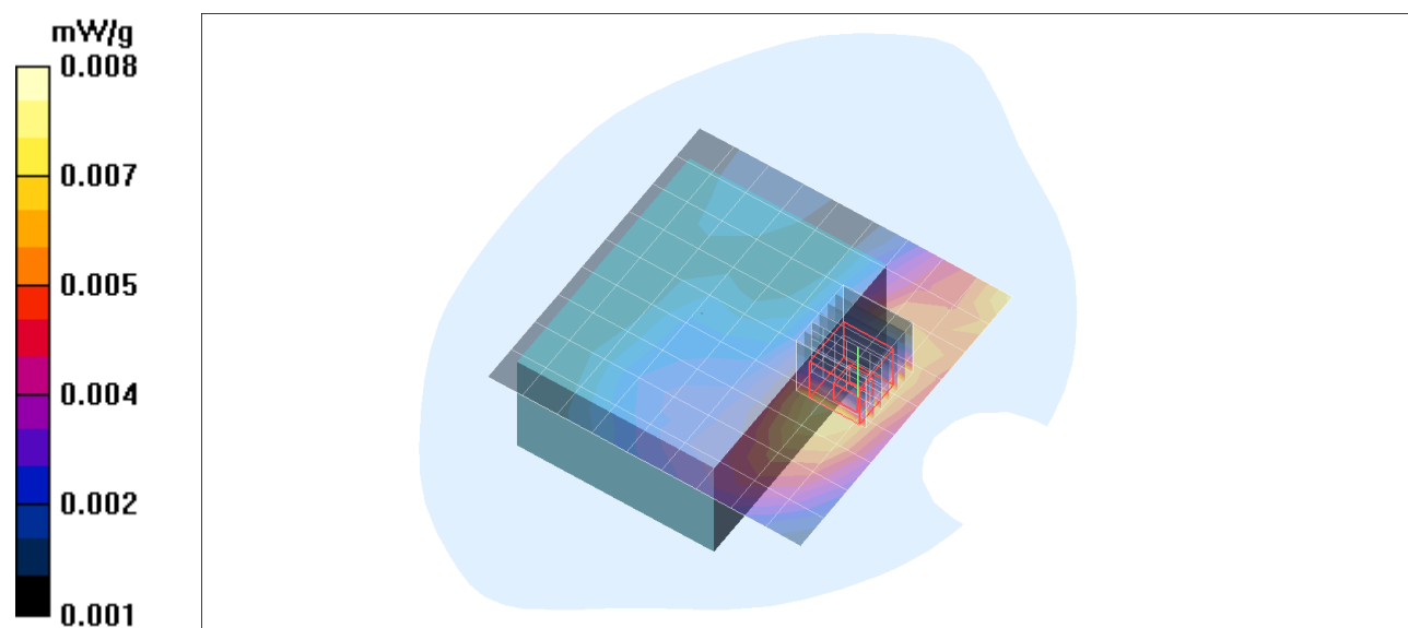
Plot. 4: SAR distribution plot for left side of DUT towards the flat phantom.
