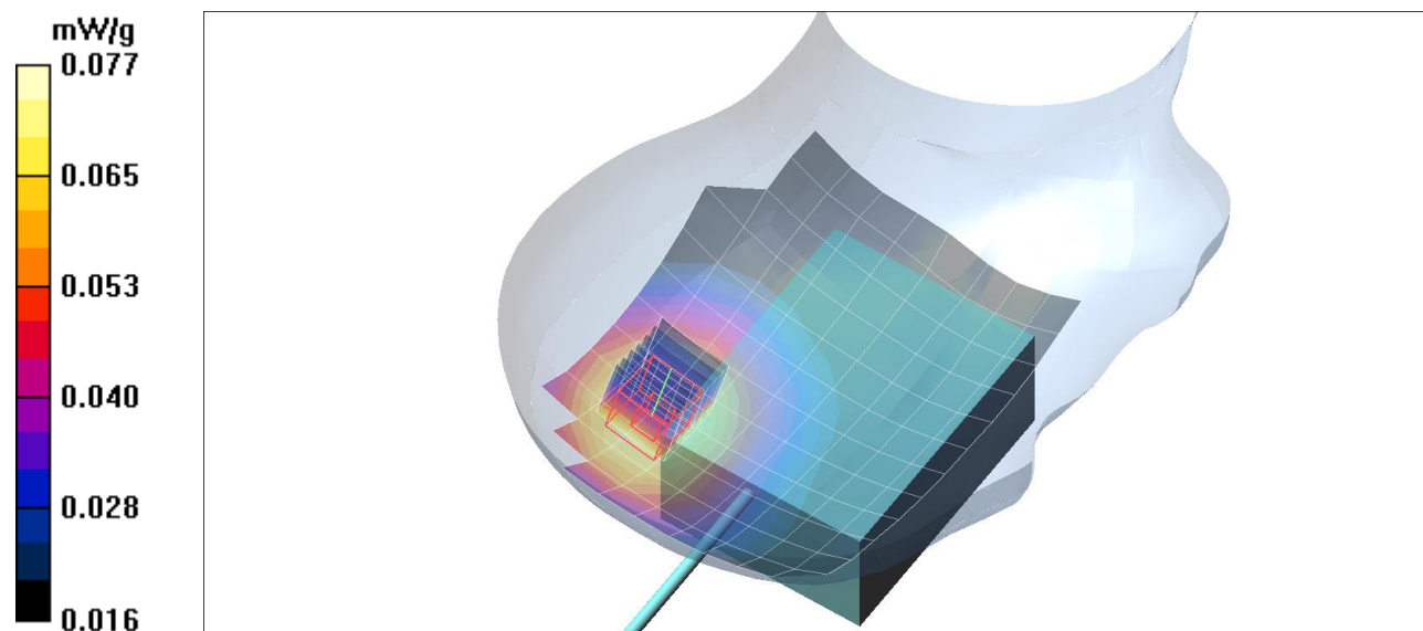
Plot. 1: SAR distribution plot for left side of DUT towards the right cheek of phantom.
