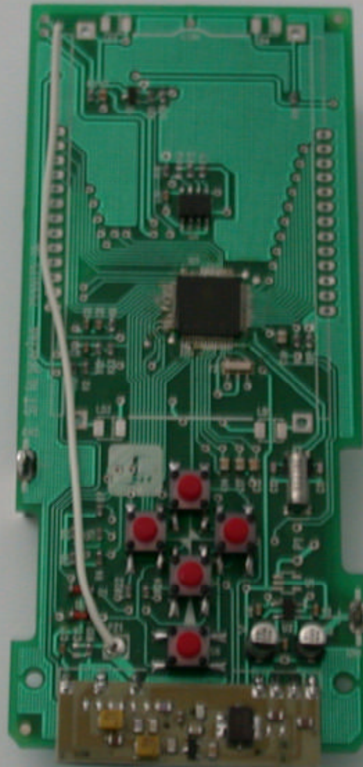
COMPONENT SIDE VIEW OF PCB WITHOUT THE LCD DISPLAY AND BACKLIGHT
