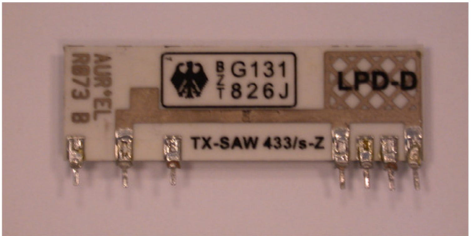
TRANSMITTER MODULE REAR VIEW
