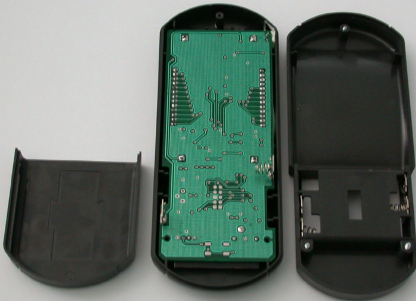
BOTTOM COVER REMOVED SOLDER SIDE VIEW OF PCB
