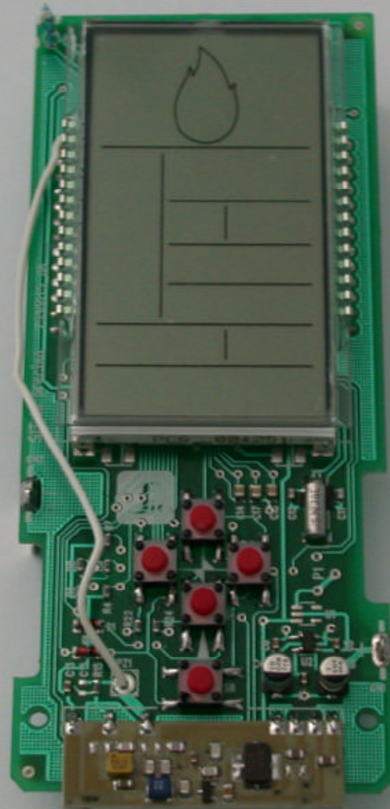
COMPONENT SIDE VIEW OF PCB
