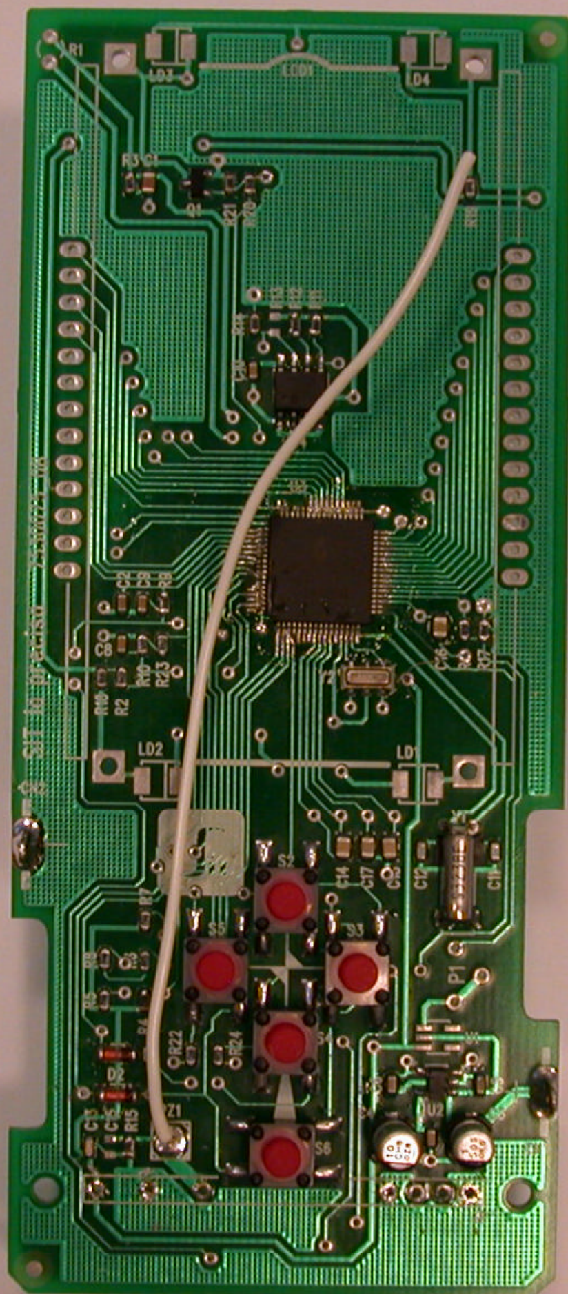
REMOTE CONTROL PCB WITHOUT THE TRANSMITTER MODULE
