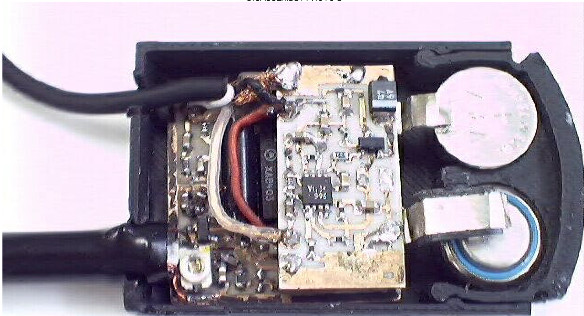
DISASSEMBLY PHOTO 1
