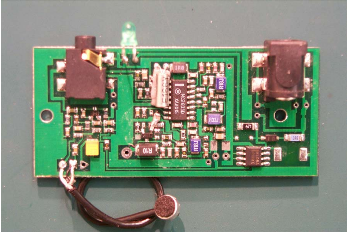
Room Monitor Model CLP-BMT2 Bottom Board
