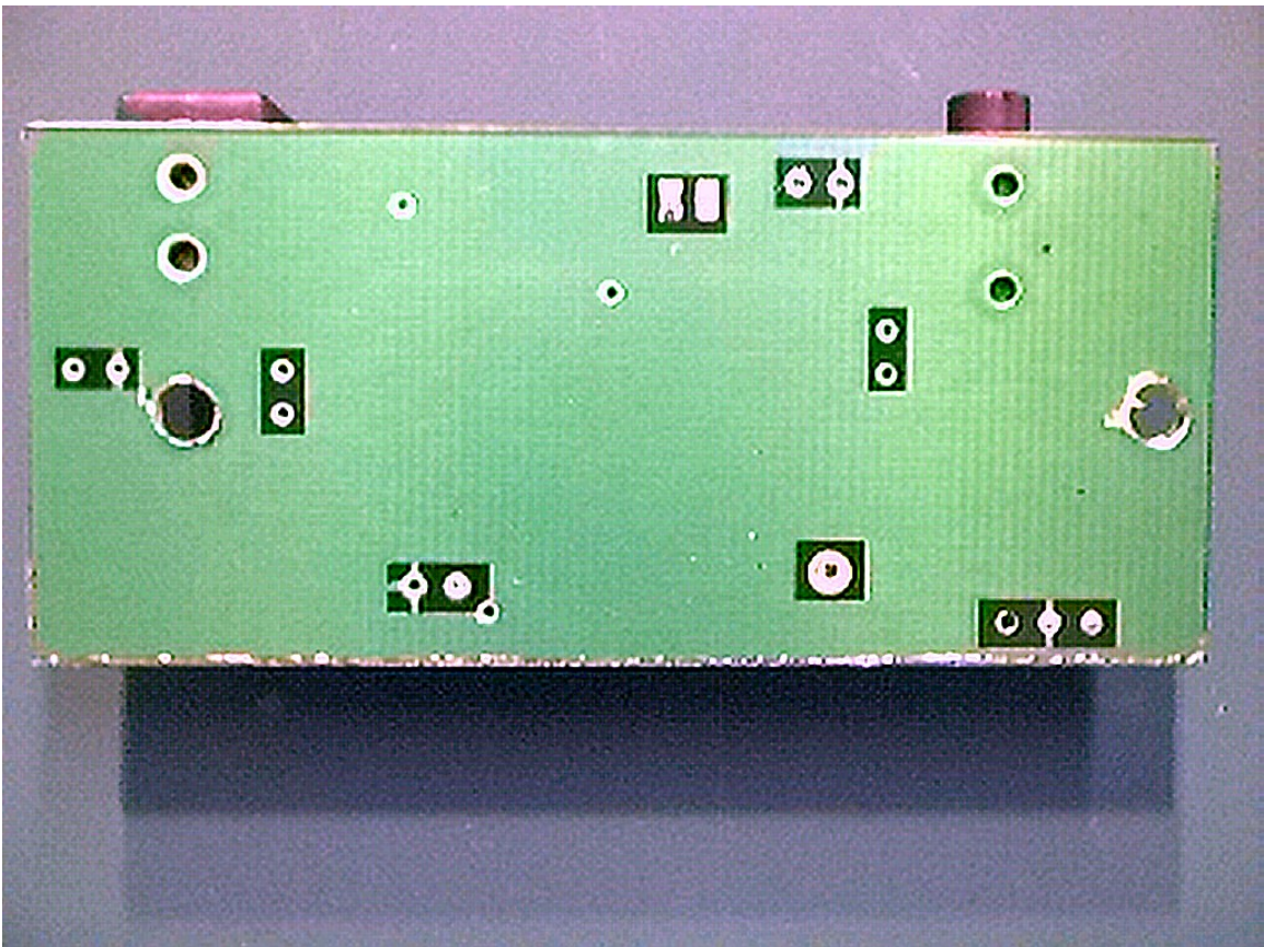
Room Monitor Model CLP-BMT1 Bottom Board
