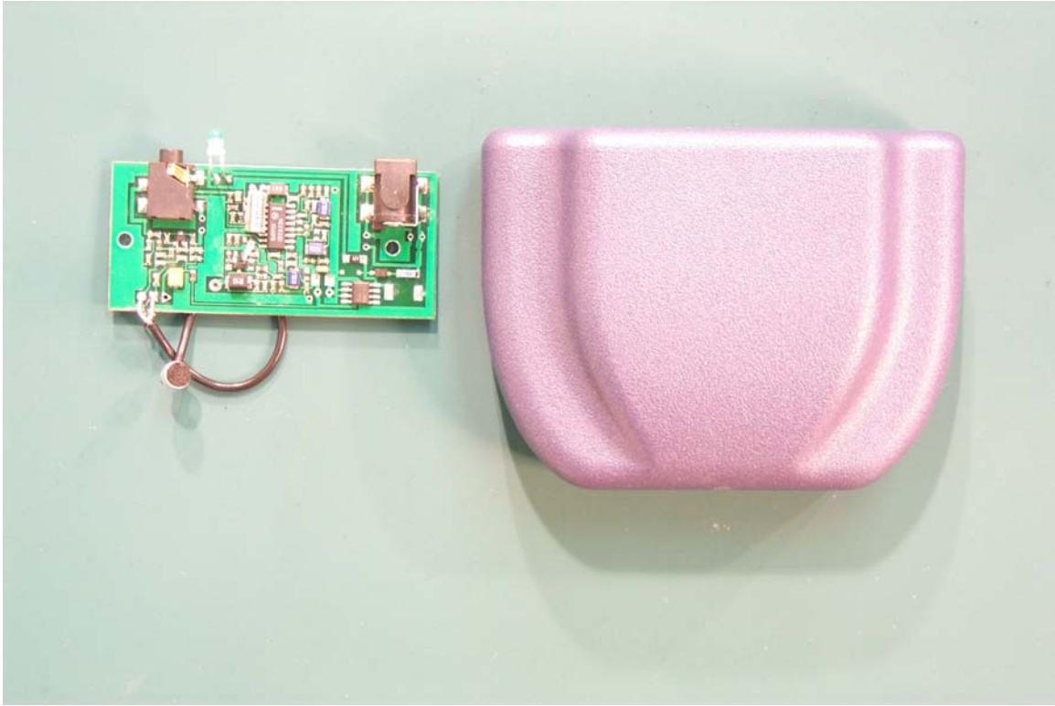
Room Monitor Model CLP-BMT1 – Board Removed from Monitor
