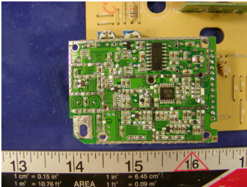
Handset Main Board Cover-Off View
