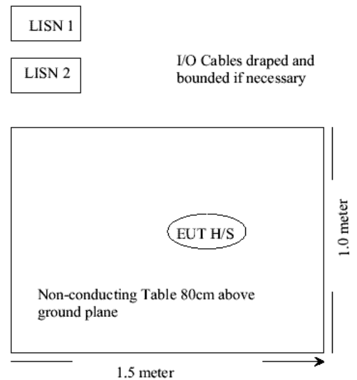
Radiated Setup for Handset
