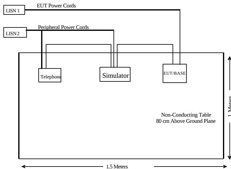
Radiated Setup for Base
